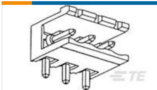
TE Part #282811-4 TERMI-BLOK HEADER ASSY90 4P.
