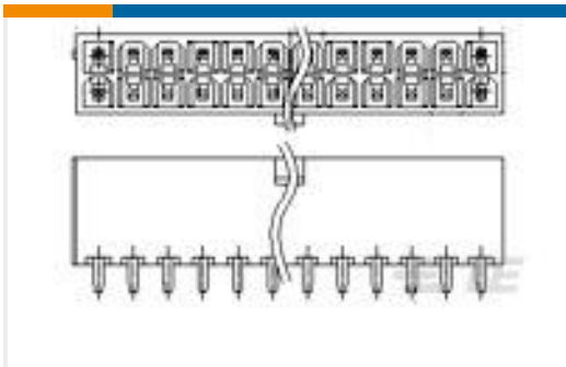
TE Part #4-1775099-8 ATX PWR CONN 24 POS
