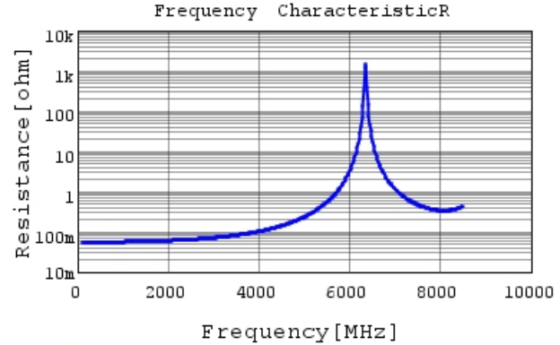
GQM22M5C2H3R9BB01 R DC0V, 25degC
