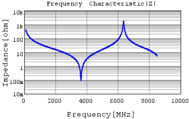
GQM22M5C2H3R9BB01 |Z| DC0V, 25degC
