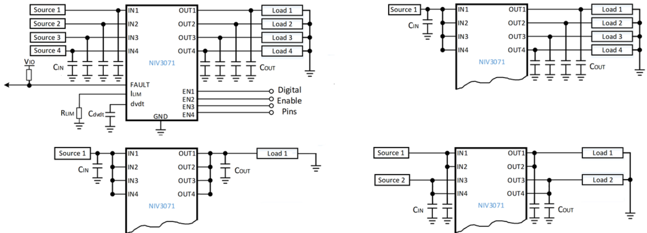
Figure 2. Application Diagrams
