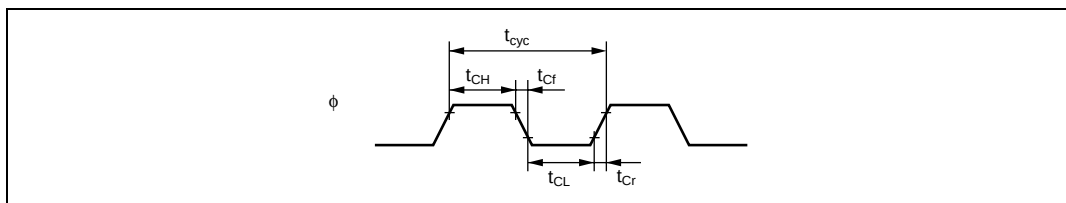
Figure 23.2 System Clock Timing
