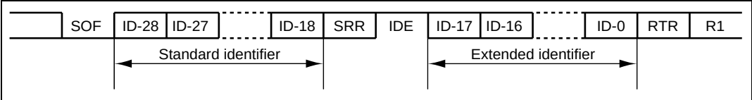
Figure 15.4 Extended Format
