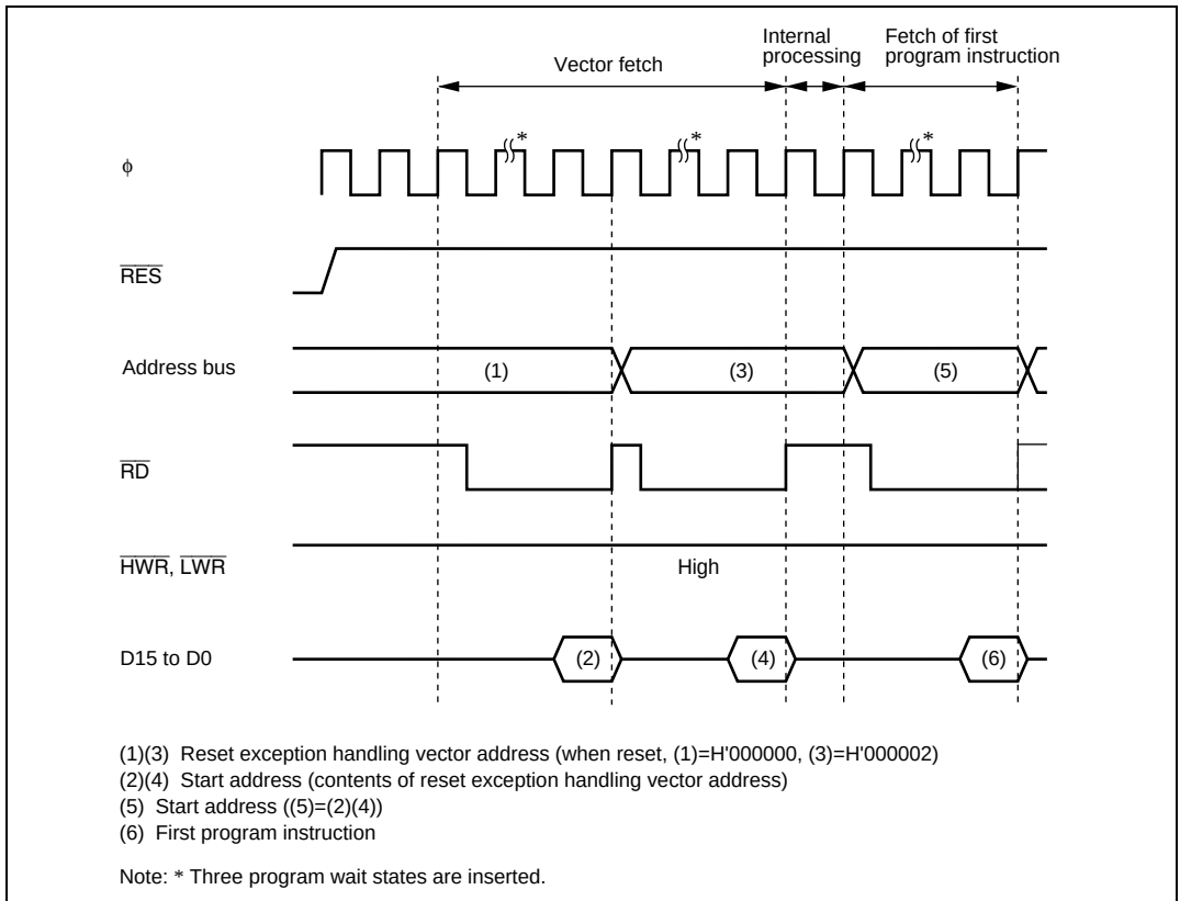
Figure 4.2 Reset Sequence (Advanced Mode with On-chip ROM Disabled: Not Available in this LSI)
