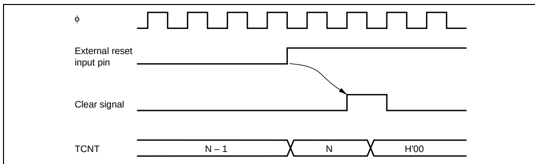
Figure 11.8 Timing of Clearing by External Reset Input
