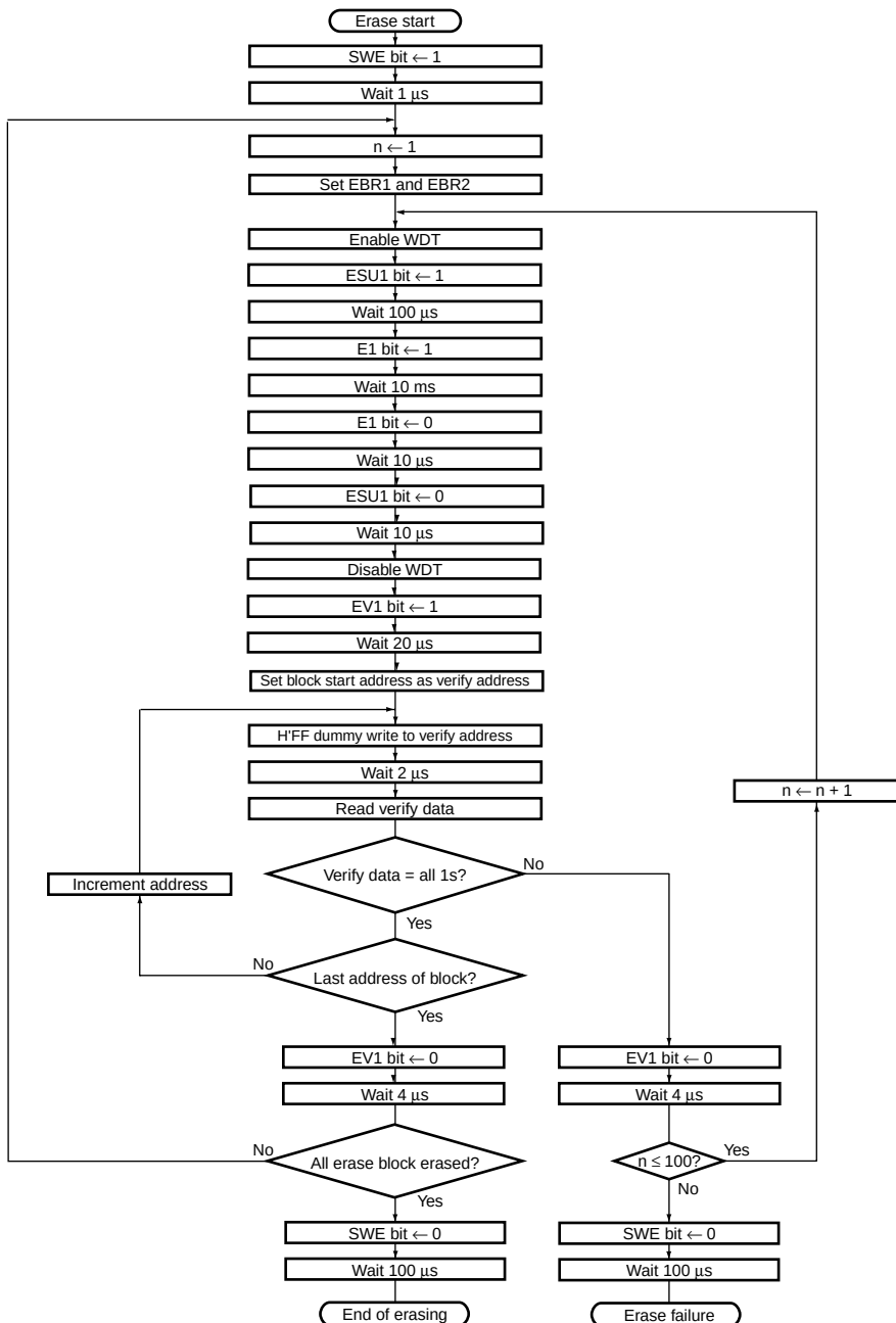
Figure 19.10 Erase/Eraser-Verify Flowchart
