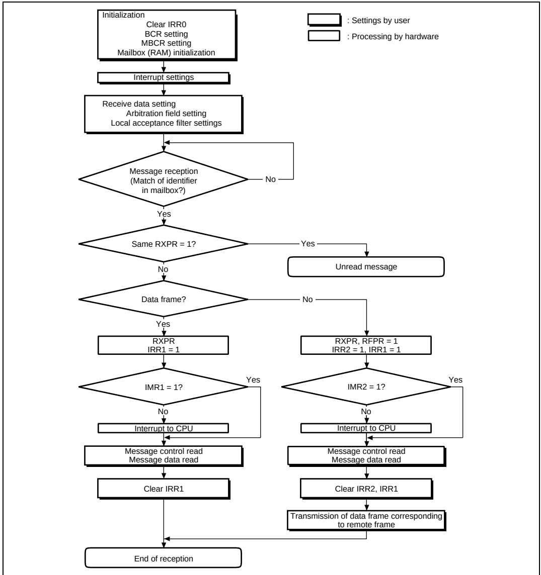
Figure 15.11 Reception Flowchart
