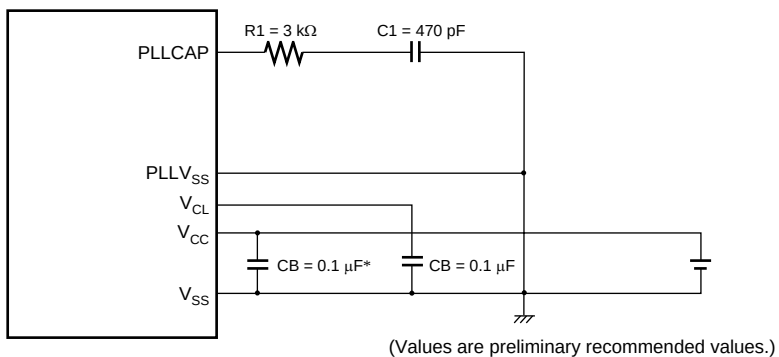
Figure 20.7 External Circuitry Recommended for PLL Circuit
