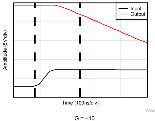
Figure 5-29. Positive Overload Recovery
