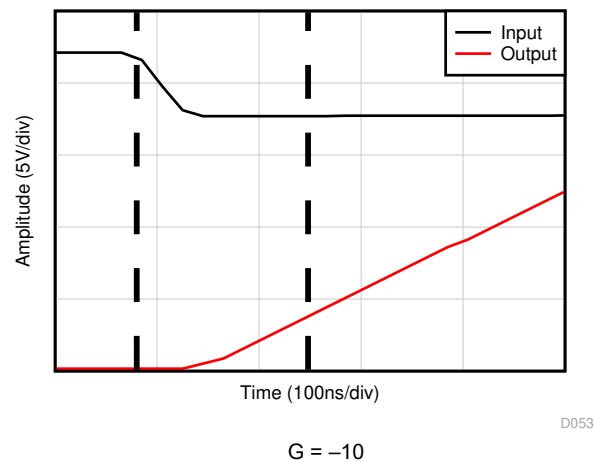
Figure 5-30. Negative Overload Recovery
