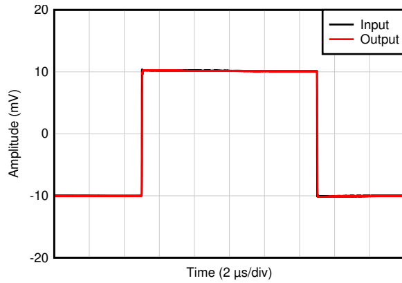
Figure 5-31. Small-Signal Step Response
