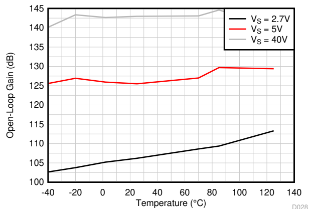
Figure 5-24. Open-Loop Voltage Gain vs Temperature (dB)
