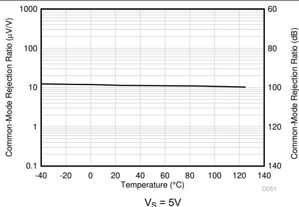
Figure 5-18. CMRR vs Temperature
