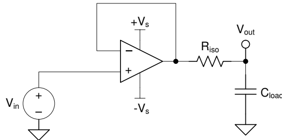
Figure 6-5. Extending Capacitive Load Drive With the TLV9361-Q1
