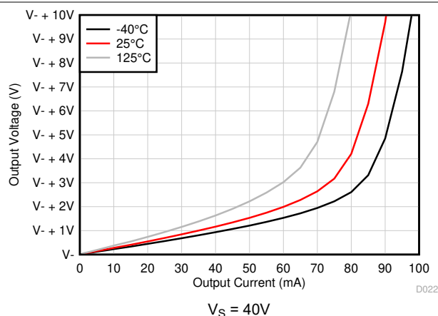
Figure 5-13. Output Voltage Swing vs Output Current (Sinking)
