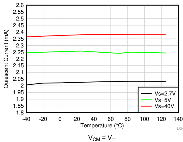
Figure 5-23. Quiescent Current vs Temperature
