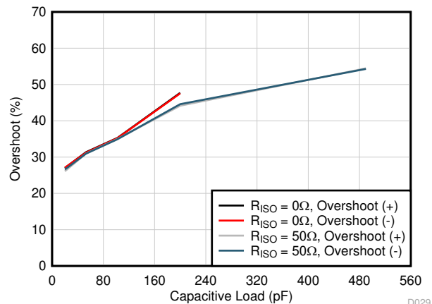
Figure 6-4. Small-Signal Overshoot vs Capacitive Load (20mV pp Output Step, G = -1 )
