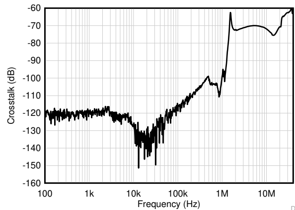
Figure 5-36. Channel Separation vs Frequency
