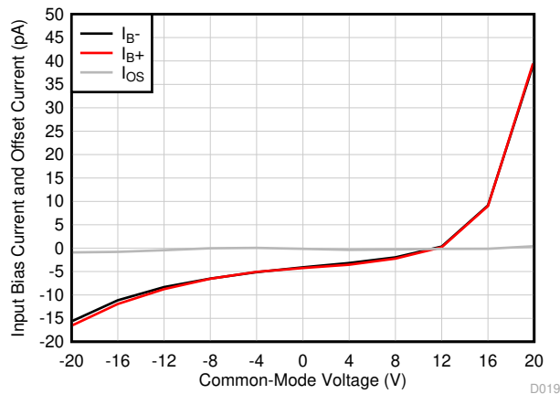
Figure 5-9. Input Bias Current and Offset Current vs Common-Mode Voltage
