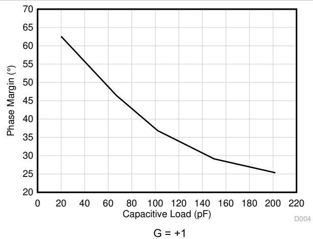
Figure 5-28. Phase Margin vs Capacitive Load
