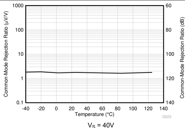
Figure 5-17. CMRR vs Temperature
