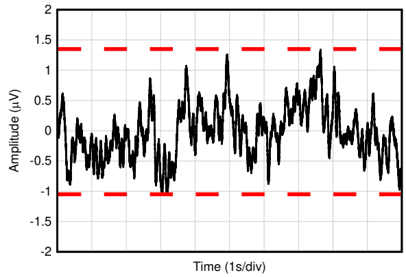
Figure 5-20. 0.1Hz to 10-Hz Noise
