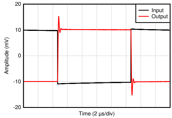
Figure 5-32. Small-Signal Step Response
