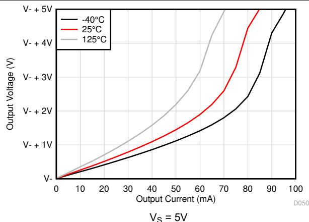
Figure 5-15. Output Voltage Swing vs Output Current (Sinking)
