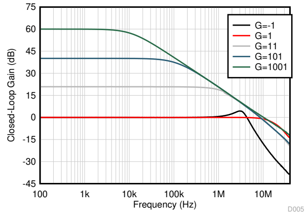
Figure 5-8. Closed-Loop Gain vs Frequency
