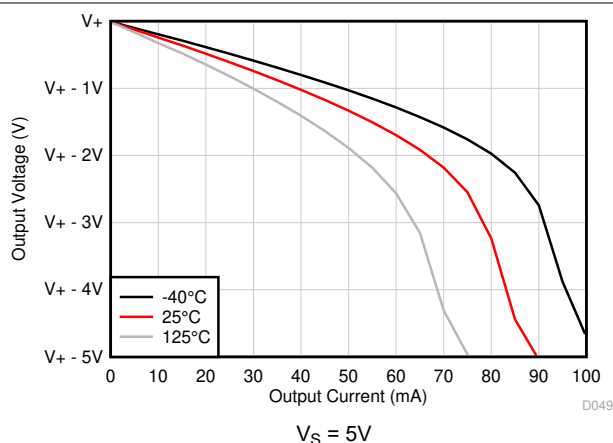
Figure 5-14. Output Voltage Swing vs Output Current (Sourcing)
