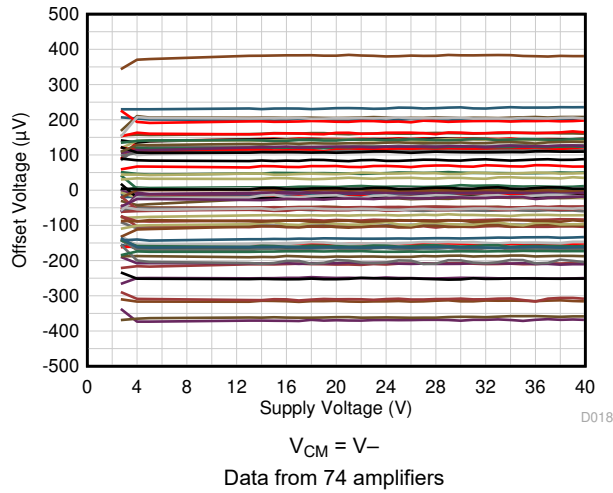
Figure 5-7. Offset Voltage vs Power Supply
