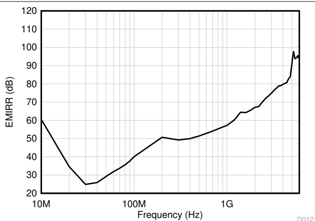
Figure 5-37. EMIRR (Electromagnetic Interference Rejection Ratio) vs Frequency
