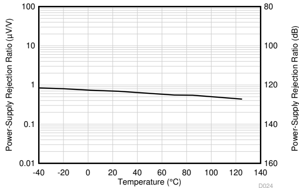
Figure 5-19. PSRR vs Temperature
