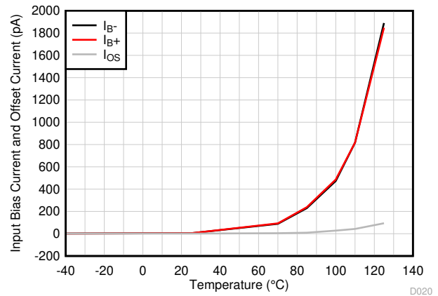
Figure 5-10. Input Bias Current and Offset Current vs Temperature
