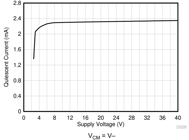
Figure 5-22. Quiescent Current vs Supply Voltage
