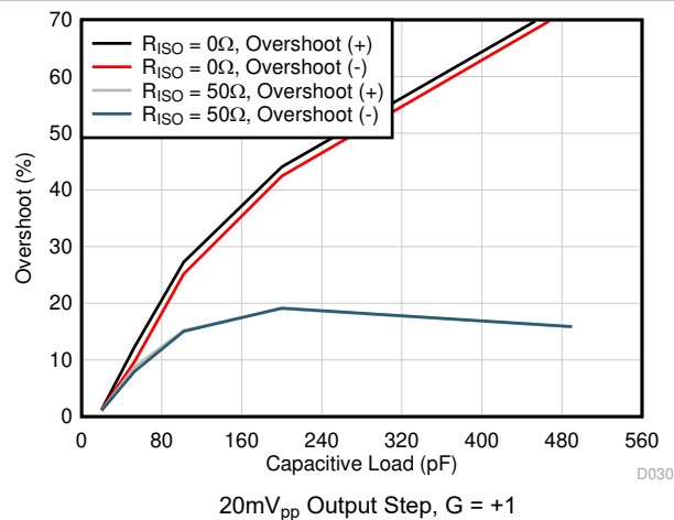
Figure 5-27. Small-Signal Overshoot vs Capacitive Load
