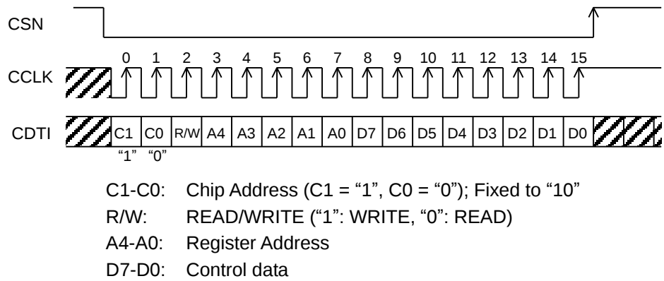
Figure 43. Serial Control I/F Timing
