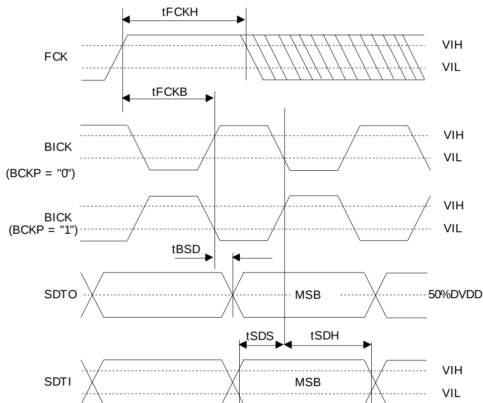
Figure 9. Audio Interface Timing (PLL Slave mode &amp; DSP mode; MSBS bit= "0")
