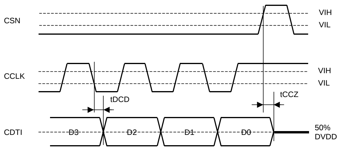
Figure 15 . Read Data Output Timing
