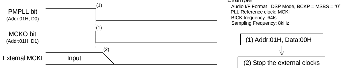
Figure 59. Clock Stopping Sequence (3)
