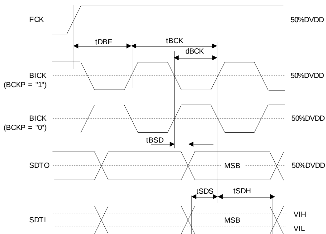
Figure 4. Audio Interface Timing (PLL/EXT Master mode &amp; DSP mode: MSBS bit = "1")
