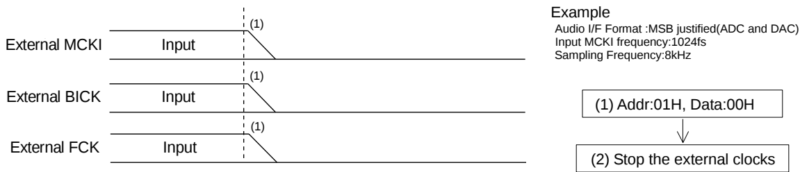
Figure 60. Clock Stopping Sequence (4)
