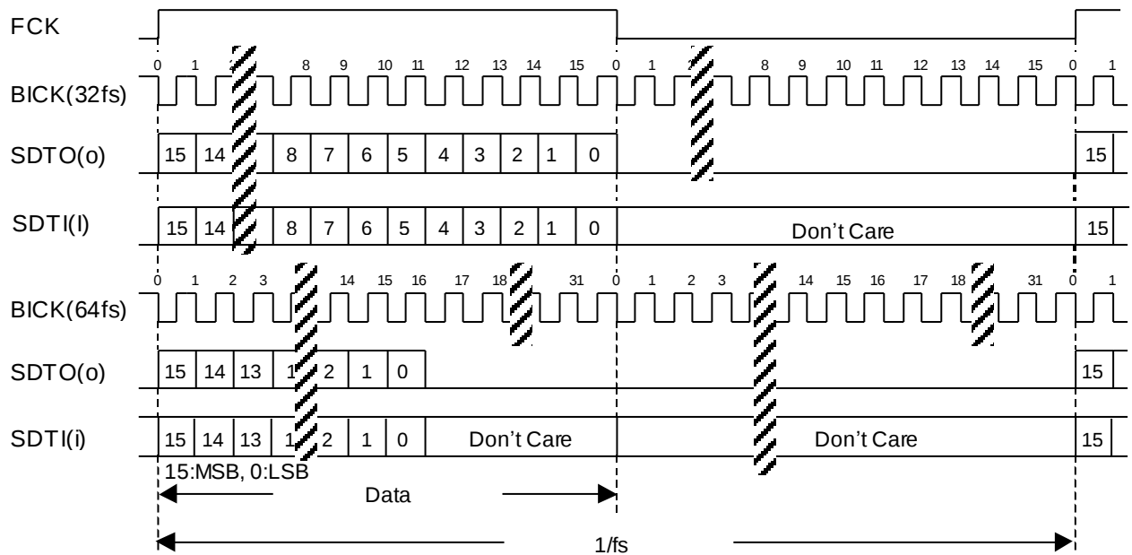
Figure 24. Mode 2 Timing
