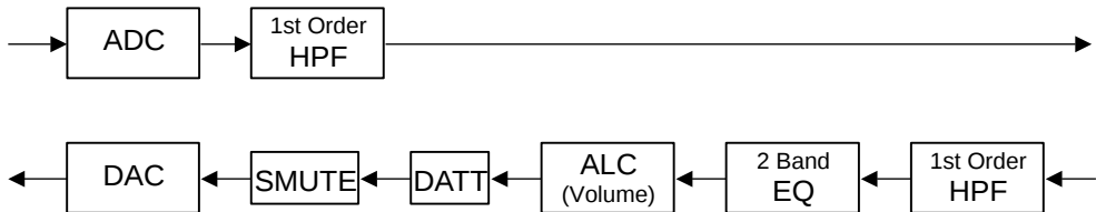
Figure 34. The path at ADCPF bit = “0”, PFDAC bit = “1” and PFSDO bit = “0”
