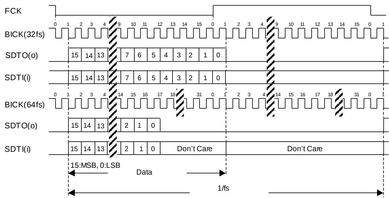
Figure 25. Mode 3 Timing
