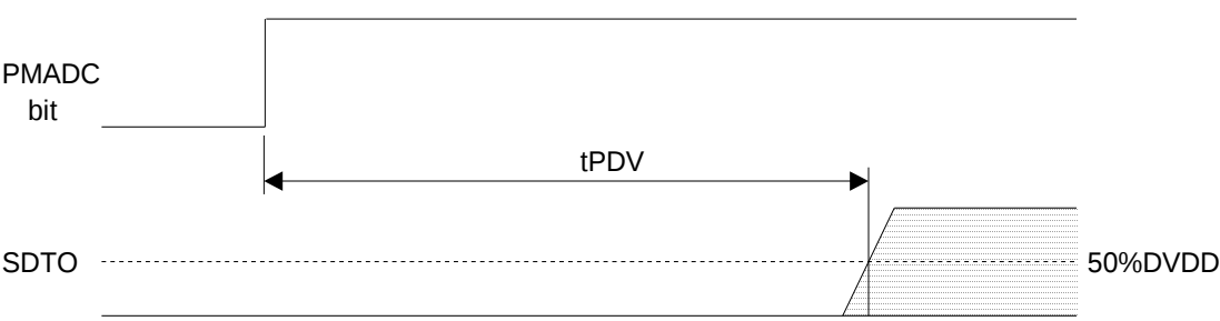
Figure 16. Power Down & Reset Timing 1
