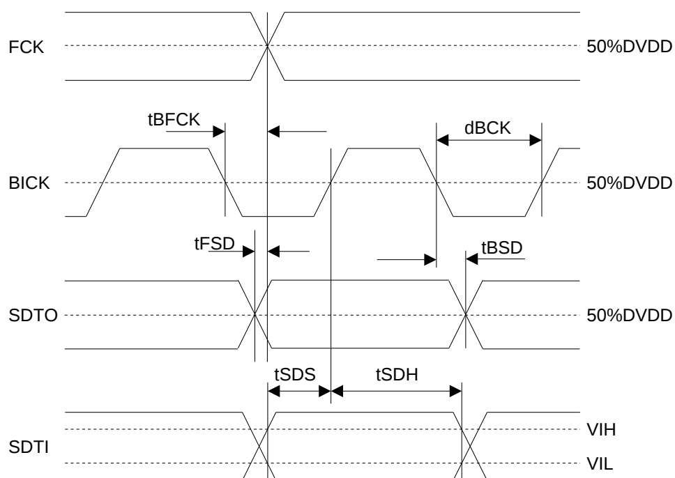
Figure 5. Audio Interface Timing (PLL/EXT Master mode &amp; Except DSP mode)
