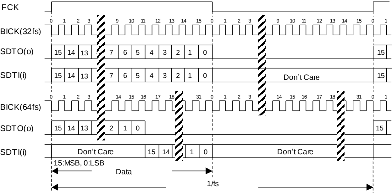
Figure 23. Mode 1 Timing
