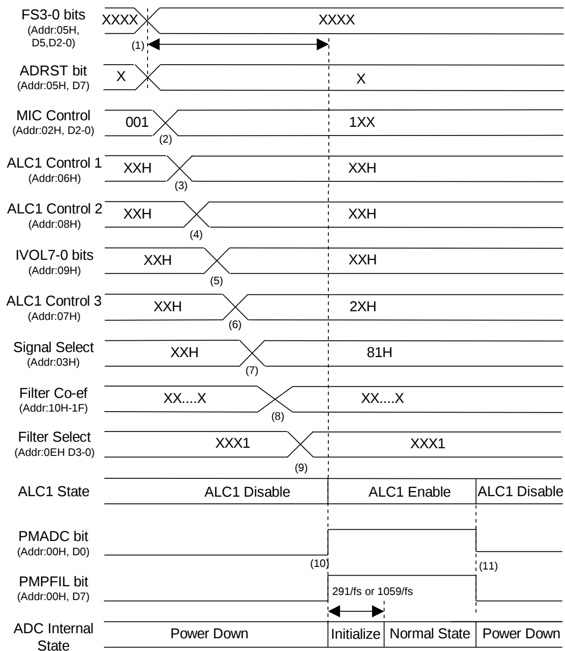
Figure 51. MIC Input Recording Sequence
