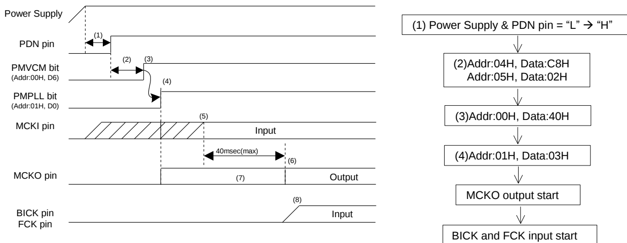
Figure 49. Clock Set Up Sequence (3)
