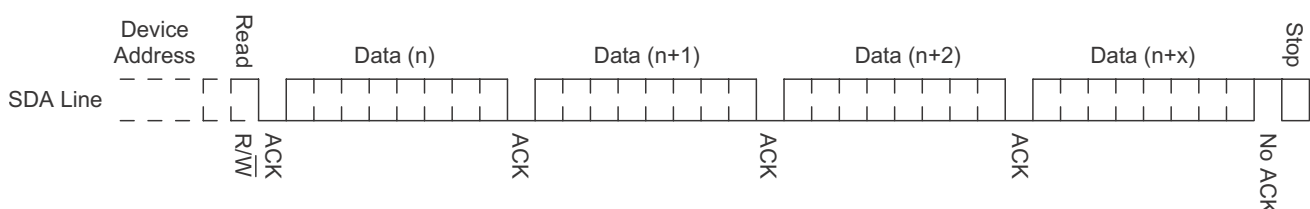
Sequential Read Timing
