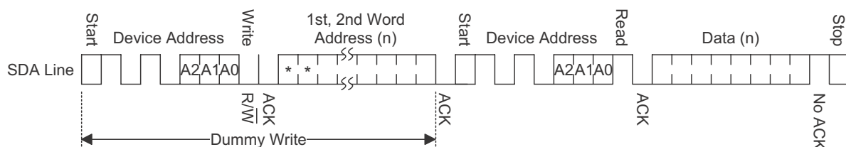
Random Read Timing
