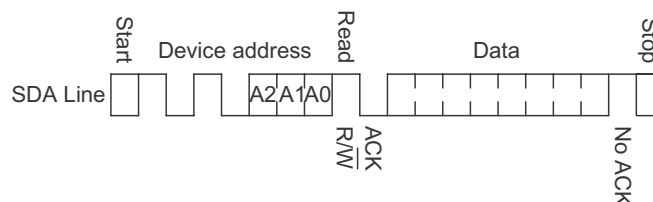
Current Read Timing
