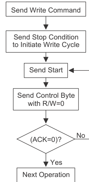
Acknowledge Polling Flow
