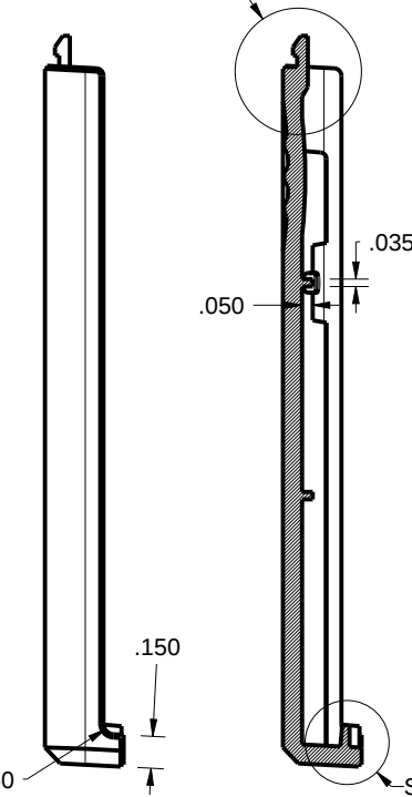
SECTION X-X
