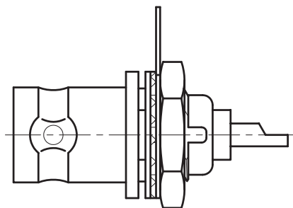
ASSEMBLY
