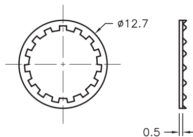
LOCK WASHER
