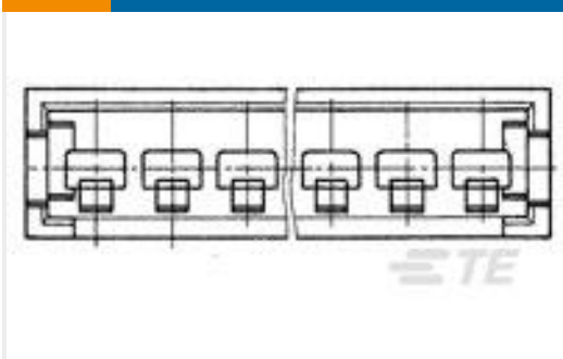
TE Part #280629 AMPMODU II COSI PIN HSG, SGL ROW, 4 POS.
