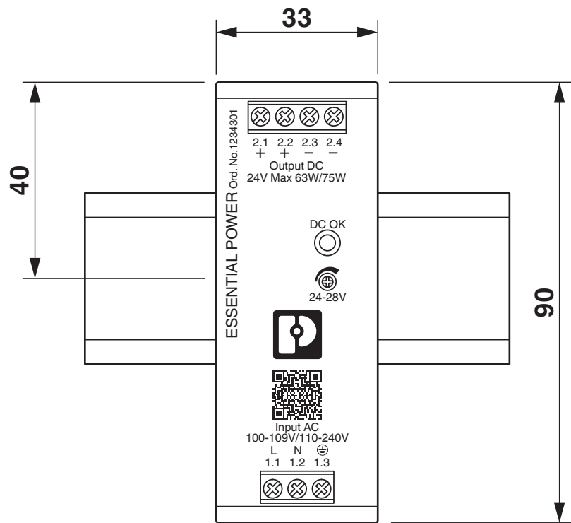
Dimensional drawing
