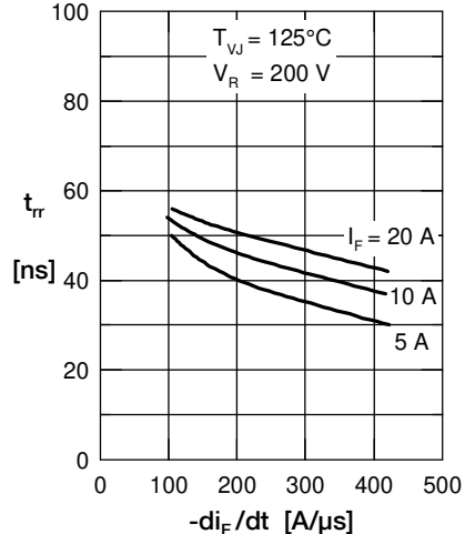
Fig. 5 Typ. reverse recov. time t_{rr} versus -di_F/dt
