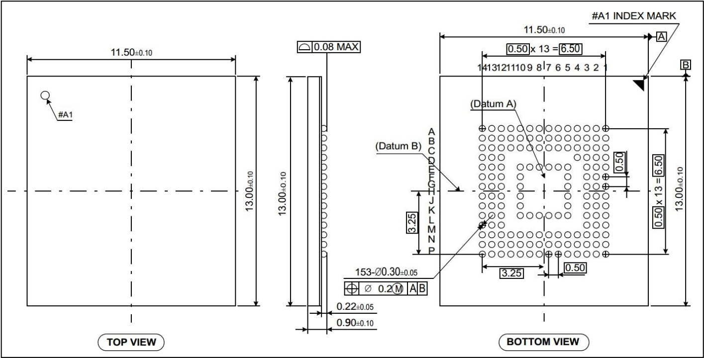
Figure 2. Package Dimension
