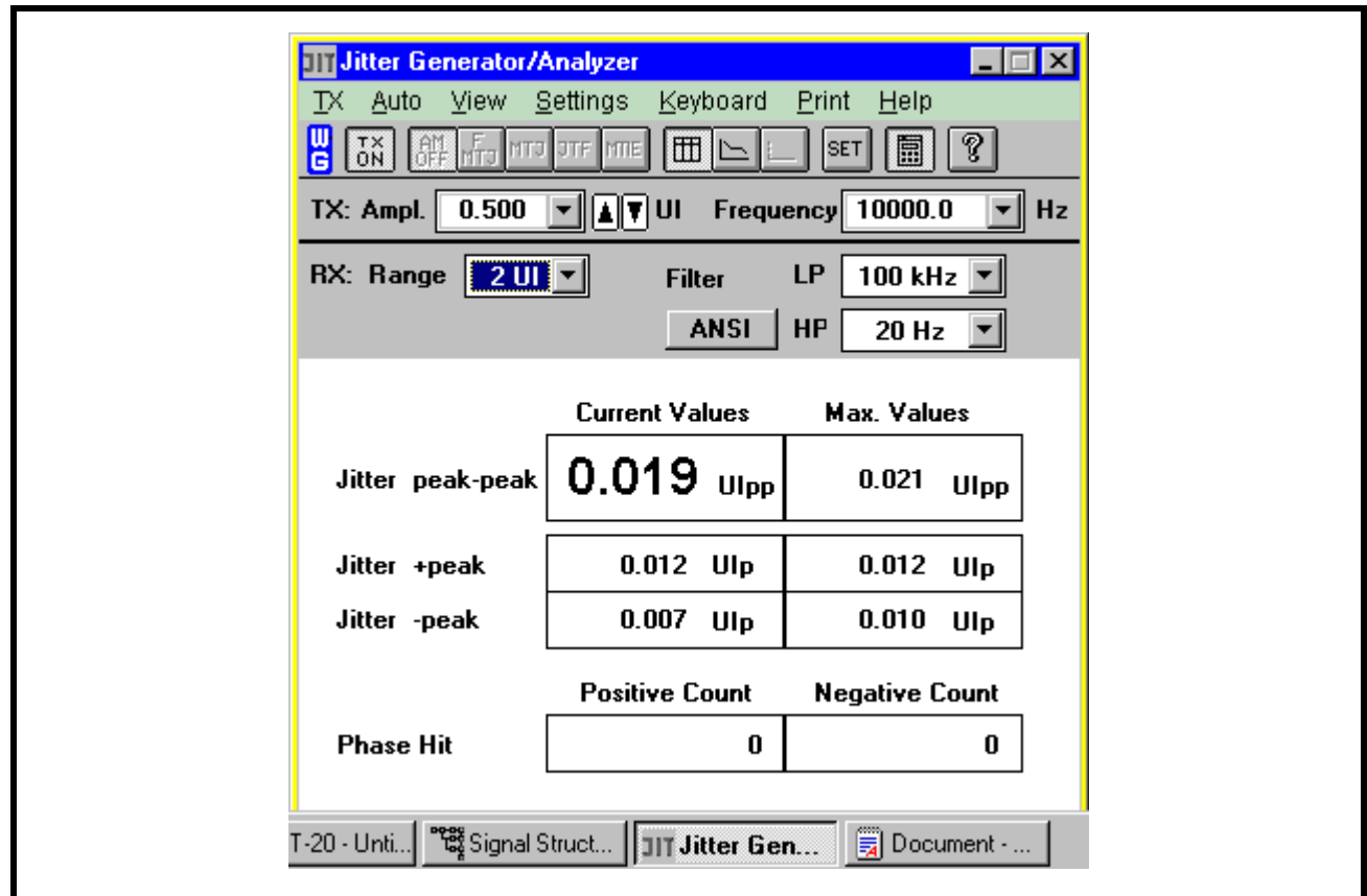
FIGURE 54. E1 INTRINSIC JITTER - MAX. VALUE MEASURED .023UIPP
