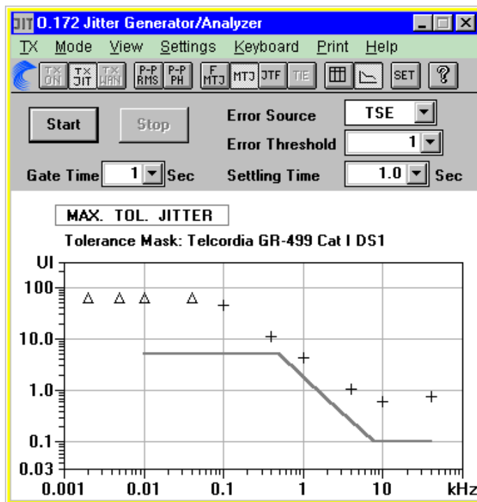
FIGURE 36. DS-1 JITTER TOLERANCE
