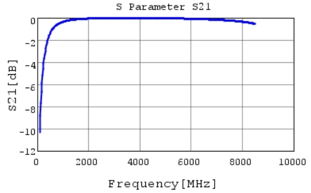
GCQ1555C1H5R1CB01 S21 DCOV, 25degC
