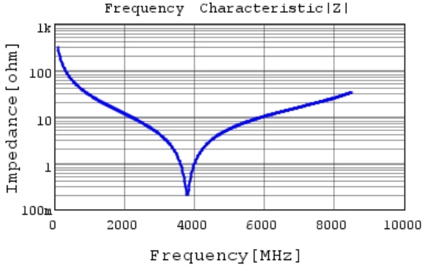
GCQ1555C1H5R1CB01 |Z| DC0V, 25degC
