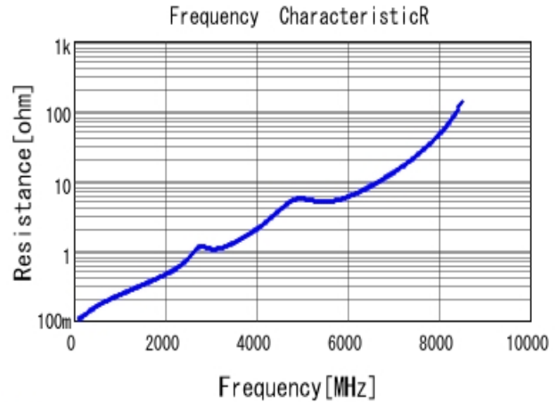
■ GCM1885C1H270JA16 R DC0V, 25degC
