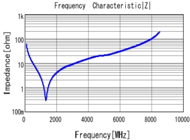
■ GCM1885C1H270JA16 |Z| DC0V, 25degC
