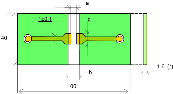
Fig.3-1 Substrate for bending test
