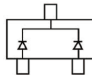
Equivalent Circuit
