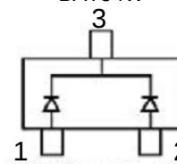
BAT54AW
