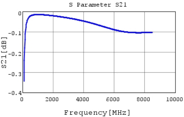
GRM0225C1A560GA02 S21 DCOV, 25degC
