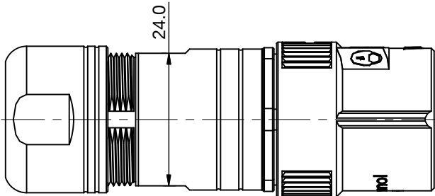
ASSEMBLED VIEW
