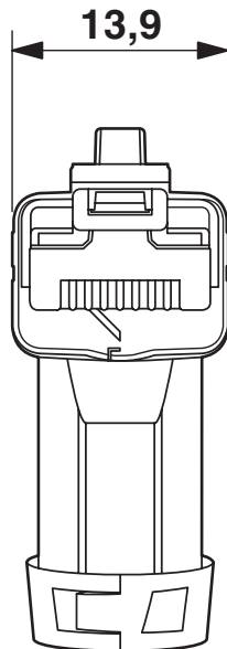
RJ45 connector, IP20, angled
