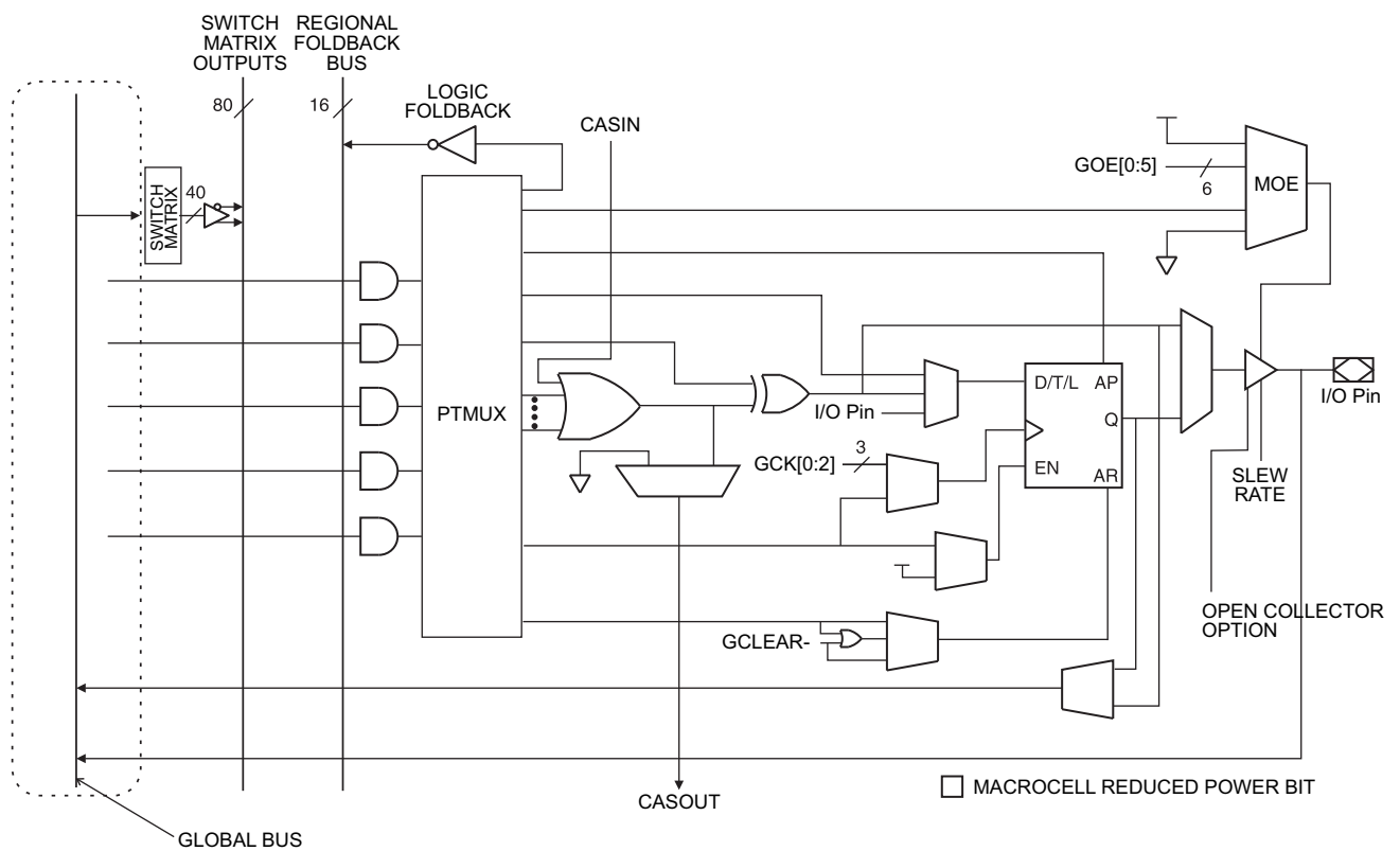
Figure 1. ATF1502AS(L) Macrocell
