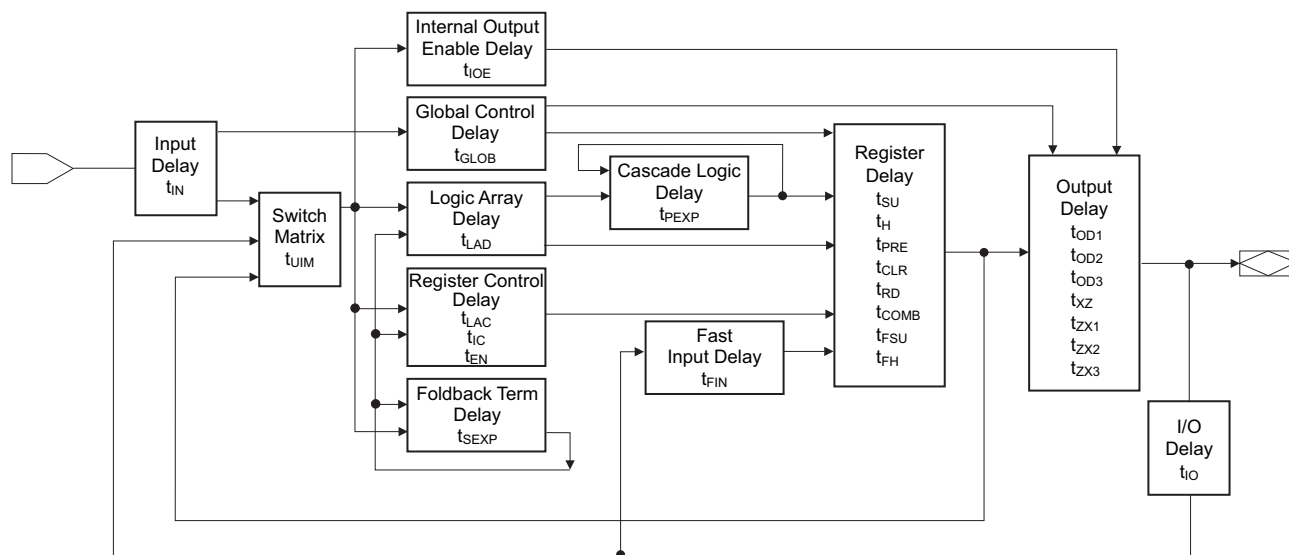
Figure 11-1. Timing Model
