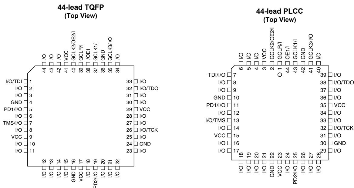
Figure 1-1. Pinouts
