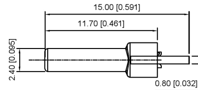
SECT B-B
