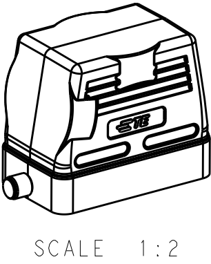
TYPE-5:H10B HOOD,LOW CONSTRUCTION, NO ENTRY,2 EAR OTHER SPEC REFER TO TYPE-1 类型-5:H10B上壳,低结构,无出线孔,2耳 其它规格尺寸参照类型-1
