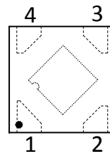
DFN1x1-4
