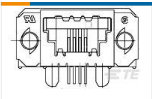
TE Part #5-1761185-3 8 SDL SE GRND RCPT ASSY
