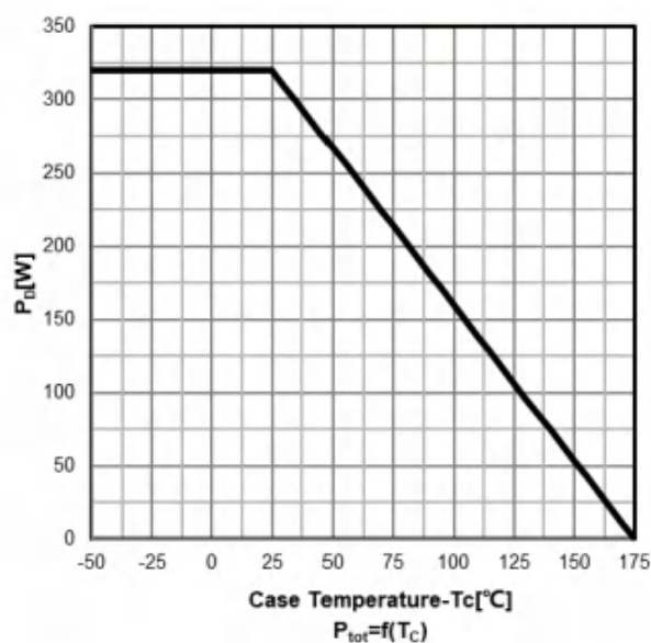
Power dissipation
