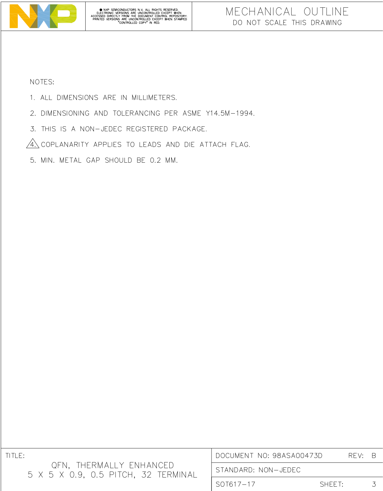
Figure 30. Package outline
