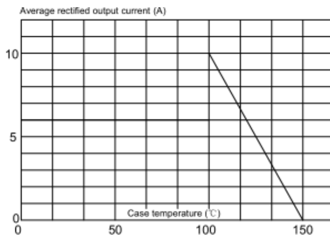
FIG.4: Average rectified output current derating curve
