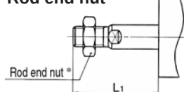
Double clevis/CQ2D
