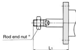
Rear flange
