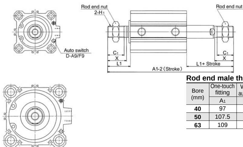
ø63 Cylinder tube form
