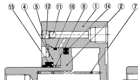
A-A section (Rod side port)
