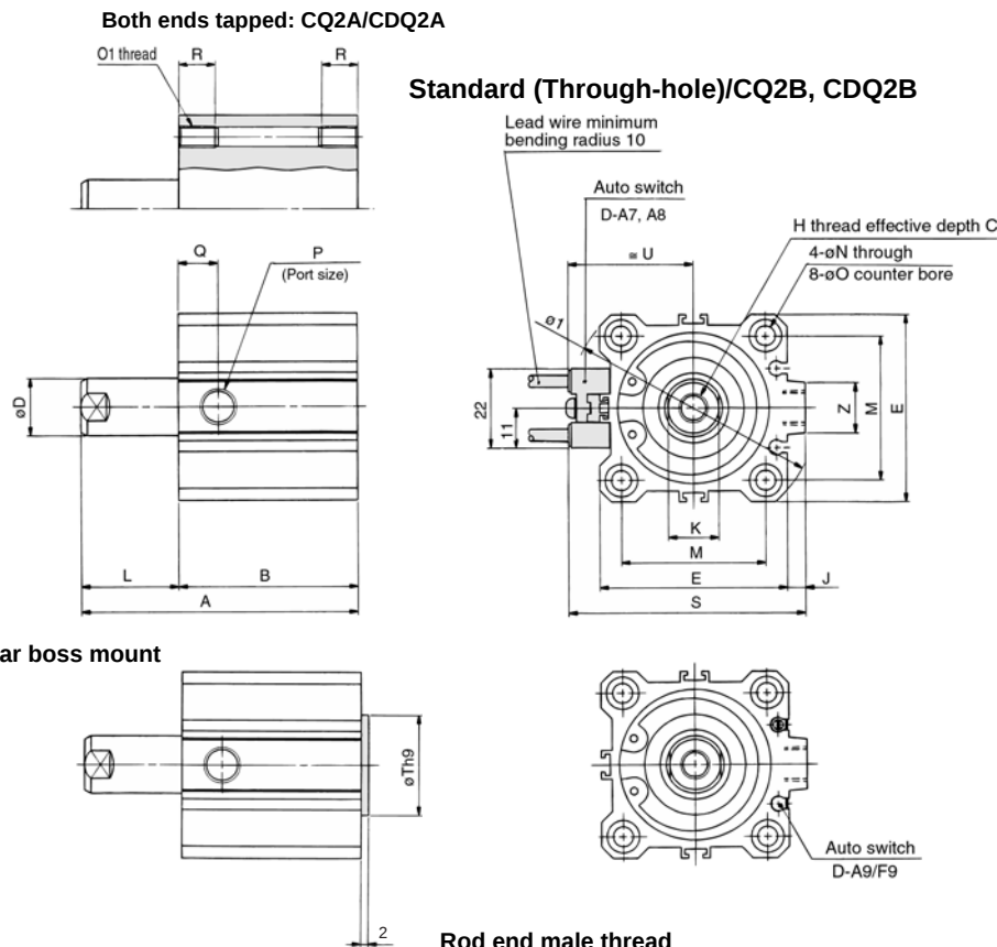
Rear boss mount (mm)
