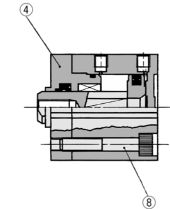
Rear boss mount
