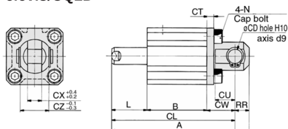
Double clevis/CQ2D
