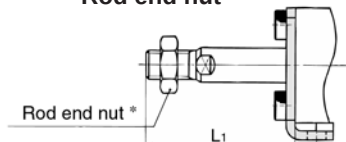
Front flange/CQ2F
