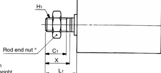
Rod end male thread (mm)
