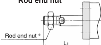
Rear flange/CQ2G
