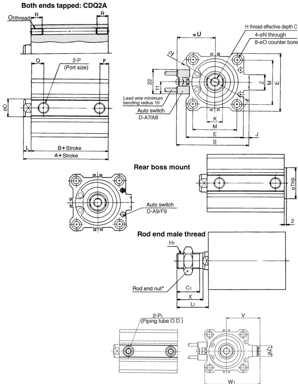
Both ends tapped (mm)
