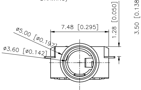
(ø3.5mm 4 POLE PLUG DETAIL DRAWING)
