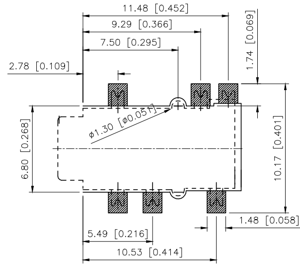
PCB LAYOUT TOP VIEW TOLERANCES:±0.05
