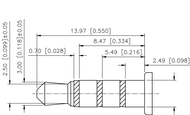
(ø3.5mm 4 POLE PLUG DETAIL DRAWING)
