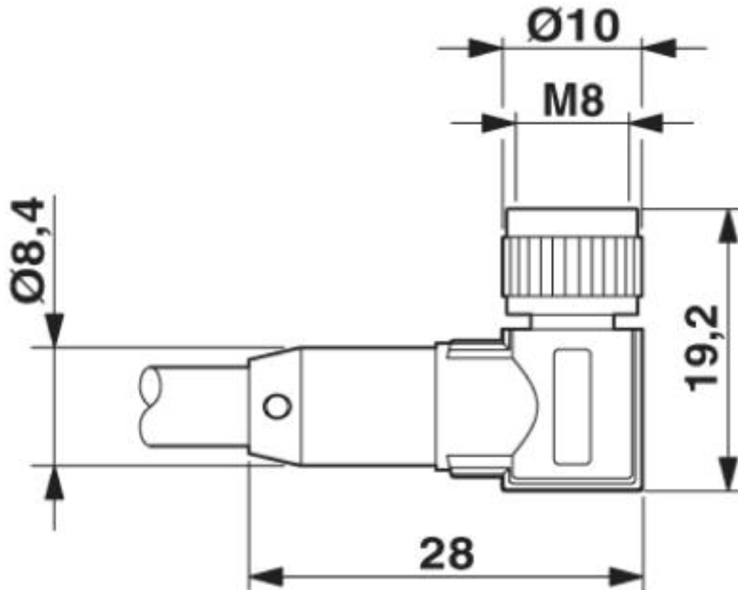
Dimensional drawing
