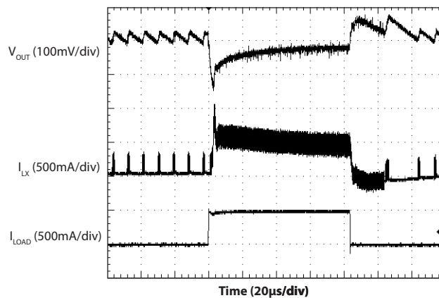
Load Transient Response — 25 to 500mA
