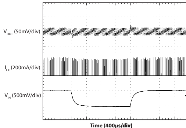
Line Transient Response — PSAVE
