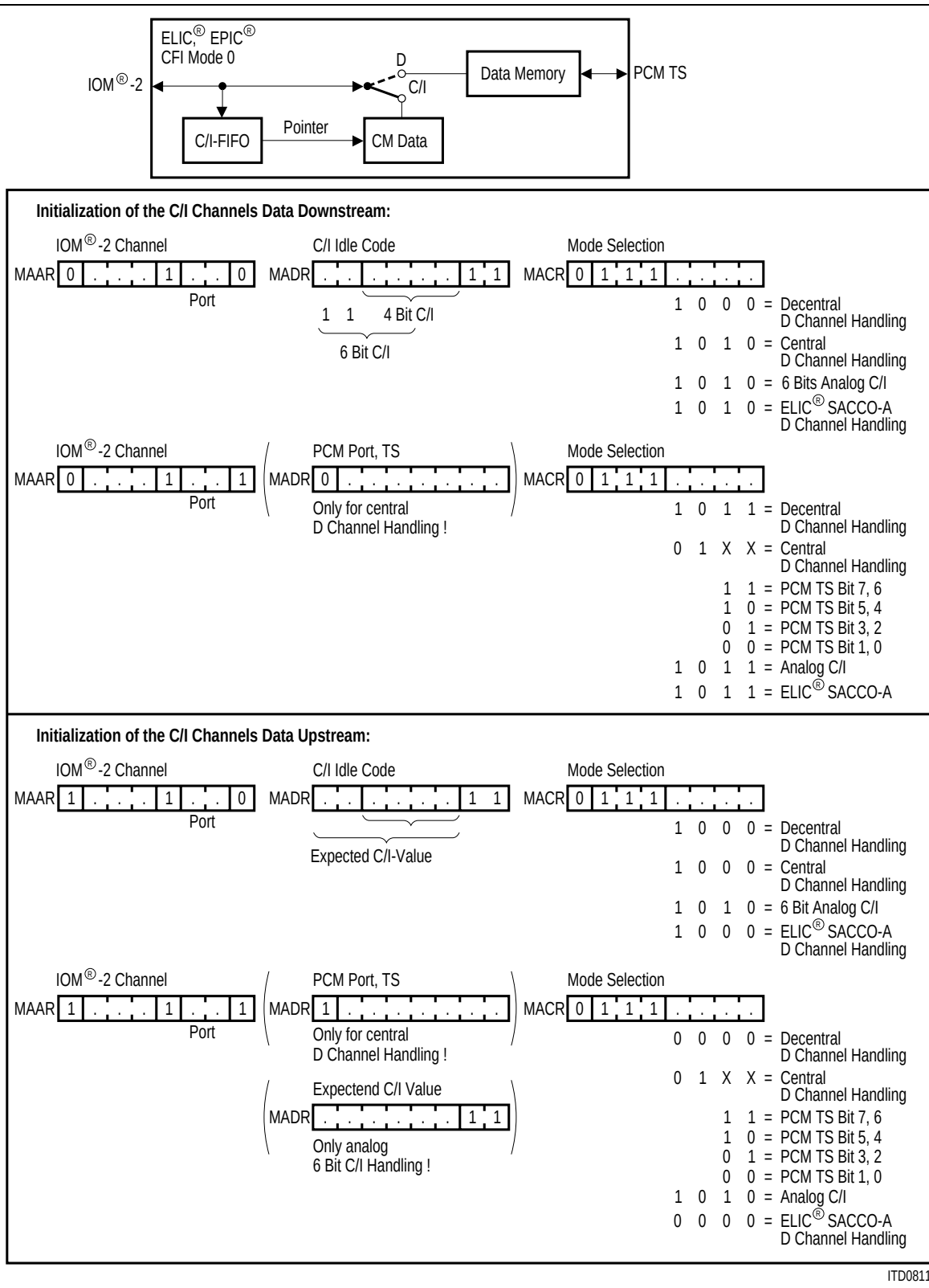
Figure 103 Preparing EPIC®s C/I Channels (working sheet)
