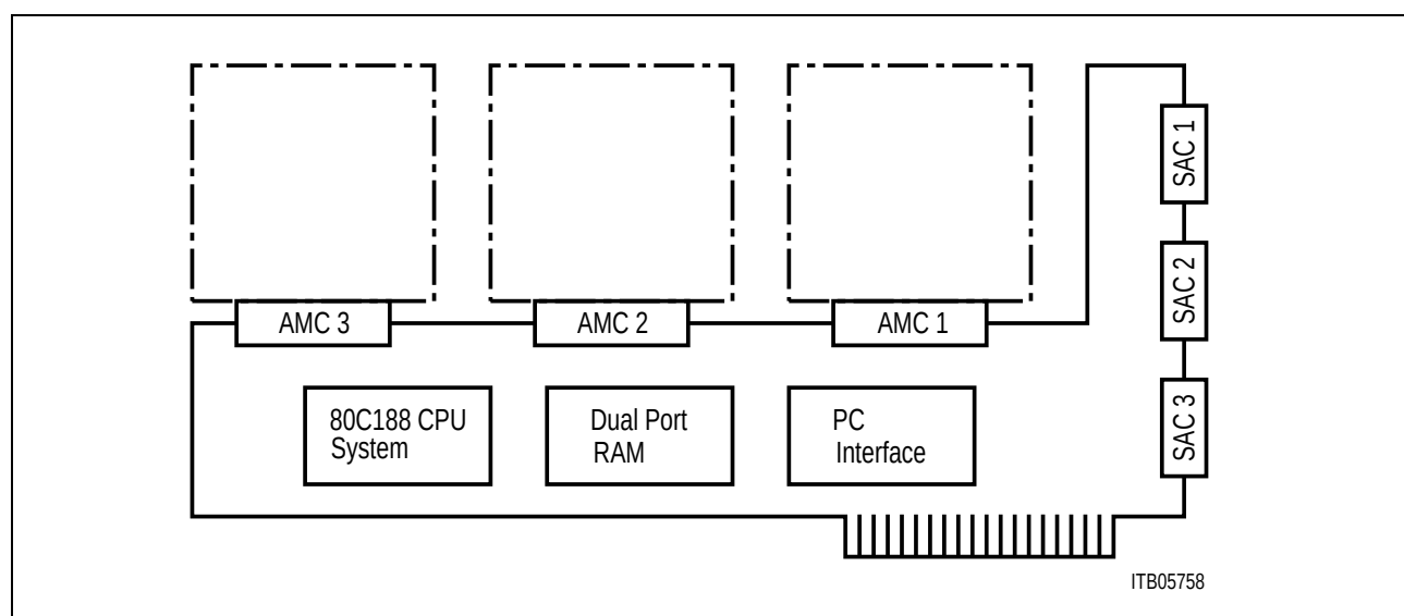
Figure 105 SIPB_5000 Mainboard
