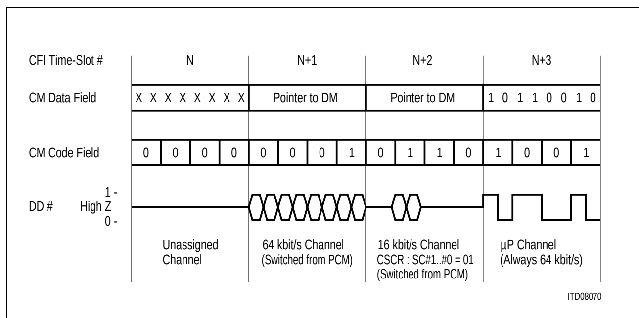
Figure 55 Tristate Behavior at the CFI
