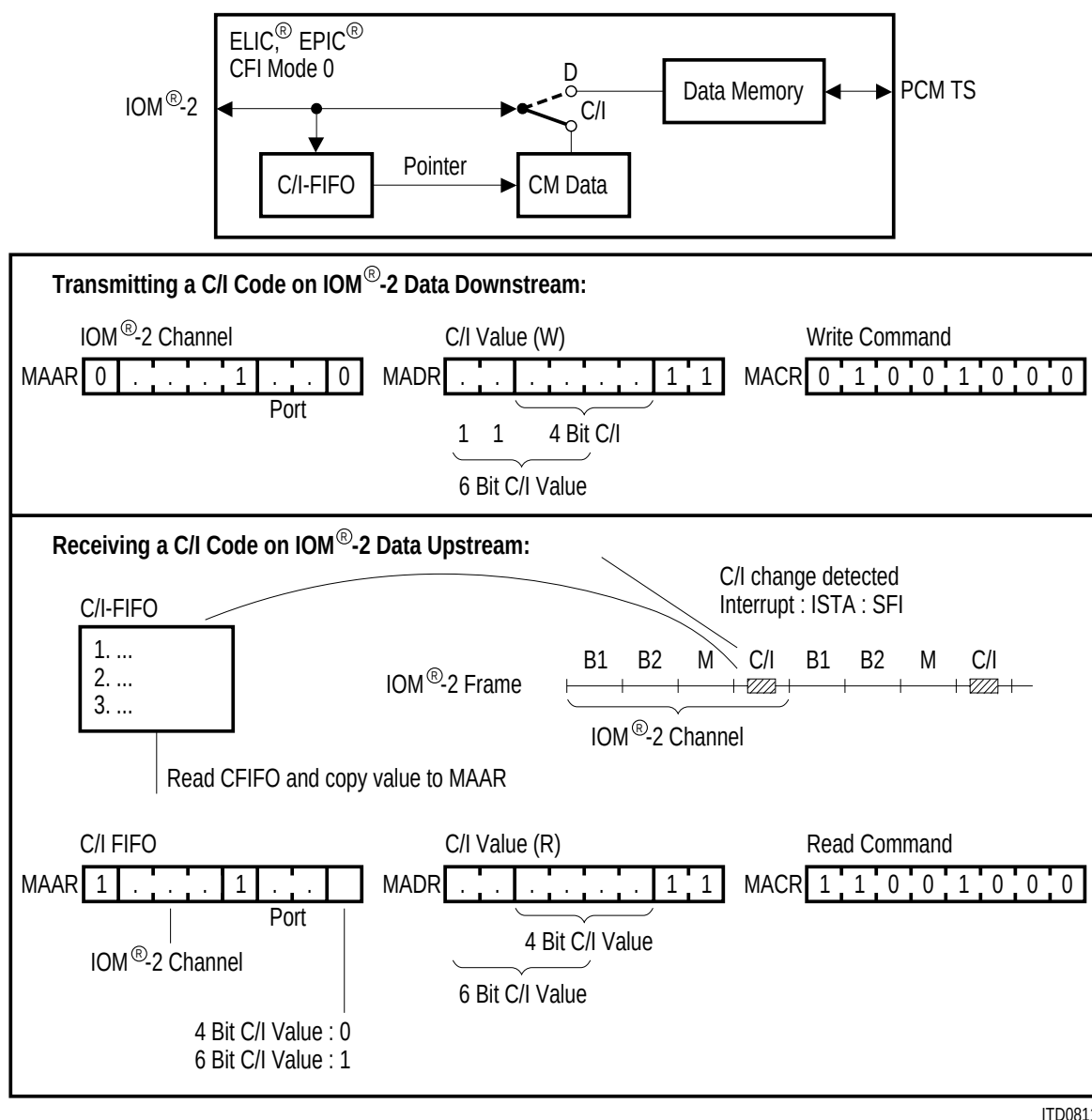
Figure 104 Receiving and Transmitting IOM ® -2 C/I-Codes (working sheet)
