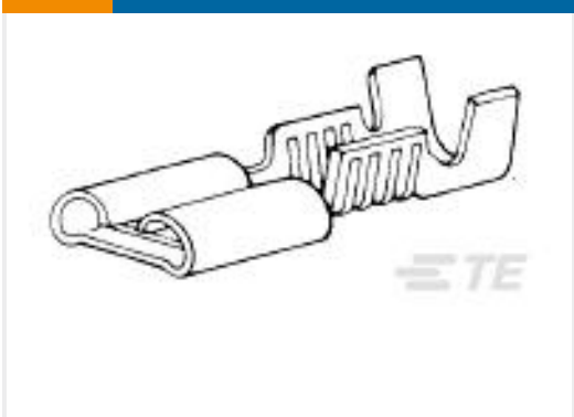
TE Part #60214-2 187 FASTON REC 20-16 AWG TPBR
