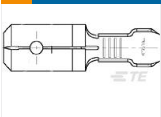
TE Part #61281-3 250 FASTON TAB 14-12 AWG TPBR
