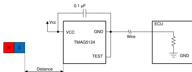
Typical Schematic
