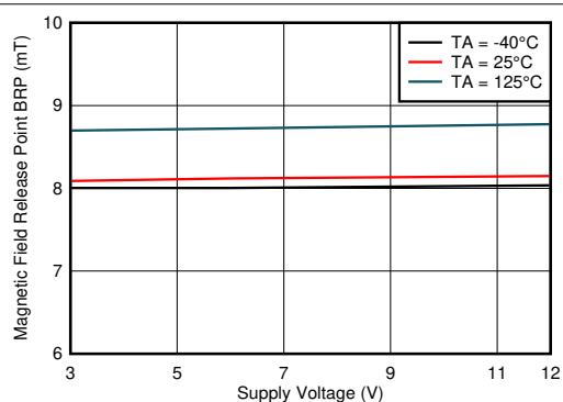
Figure 7-16. B RP vs V CC
