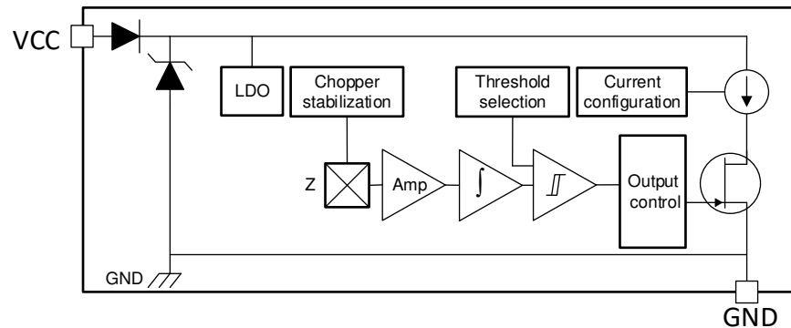
Figure 8-1. Block Diagram
