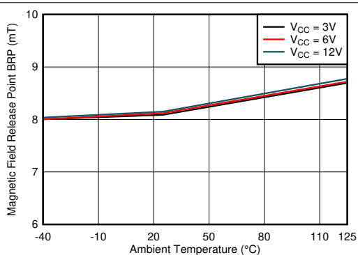
Figure 7-15. B RP vs Temperature
