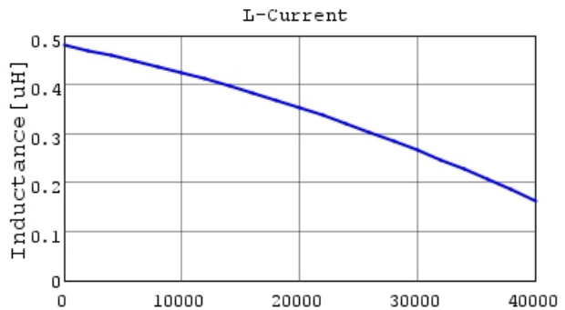
FCUL0624-H-R47M L-Current 20degC
