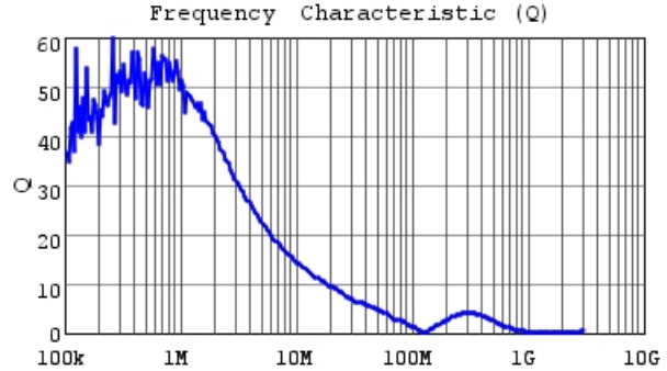
FCUL0624-H-R47M Q
