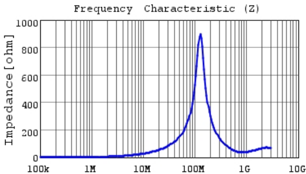
FCUL0624-H-R47M |Z|
