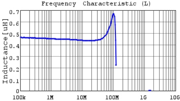
FCUL0624-H-R47M L
