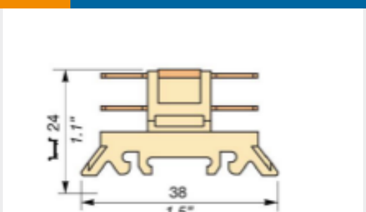
TE Part #1SNA192856R1300 H6/10.2G.2G
