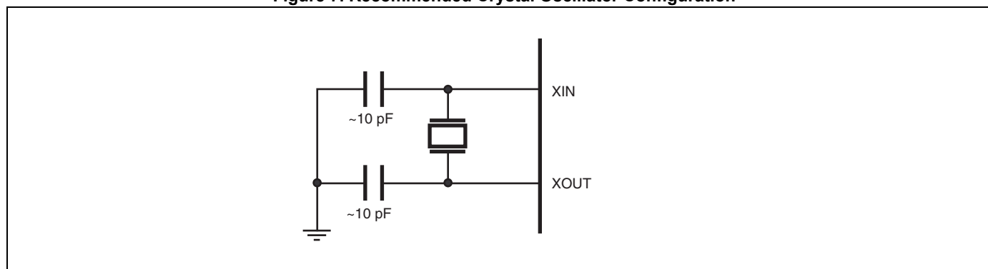
Figure 7. Recommended Crystal Oscillator Configuration
