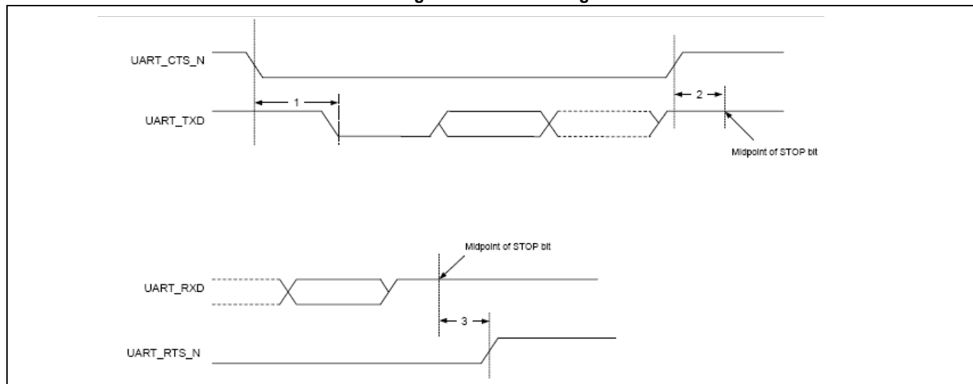
Figure 10. UART Timing
