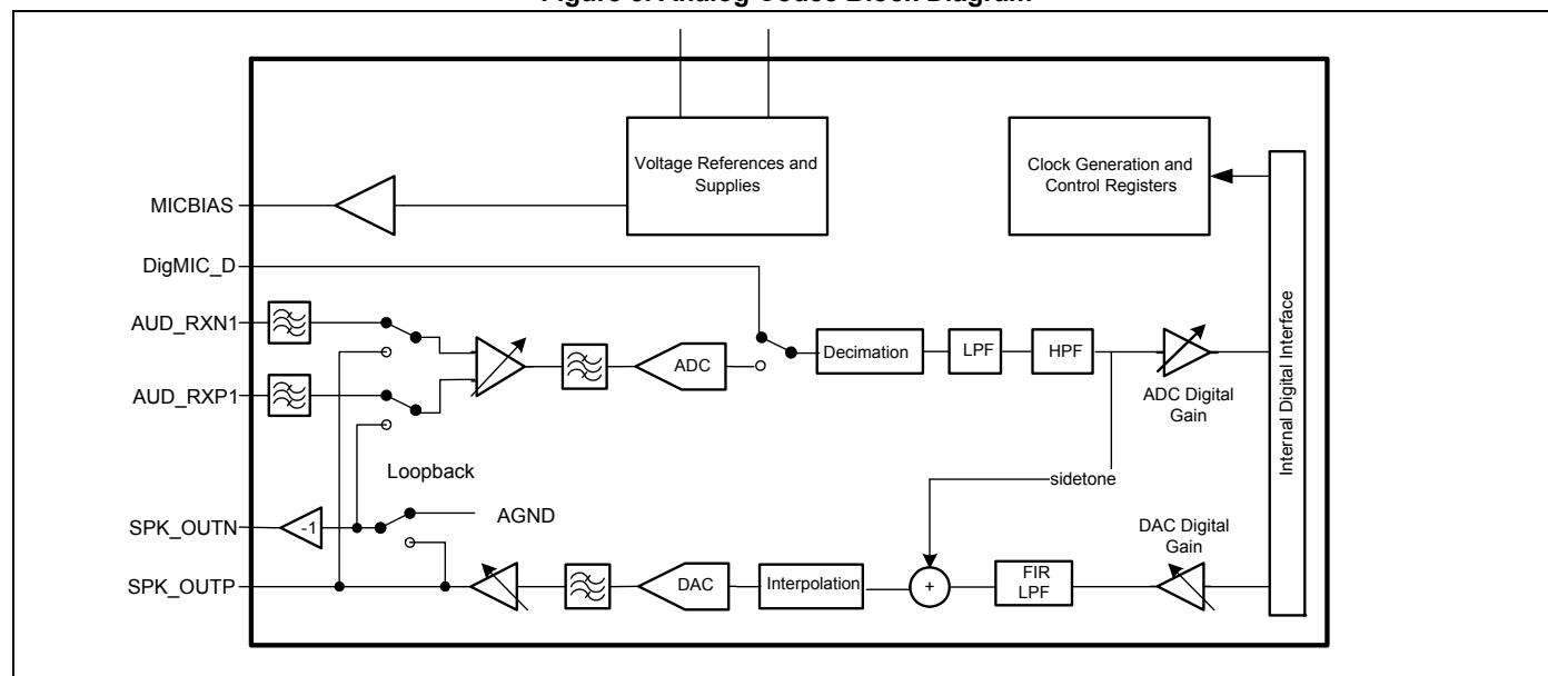
Figure 5. Analog Codec Block Diagram
