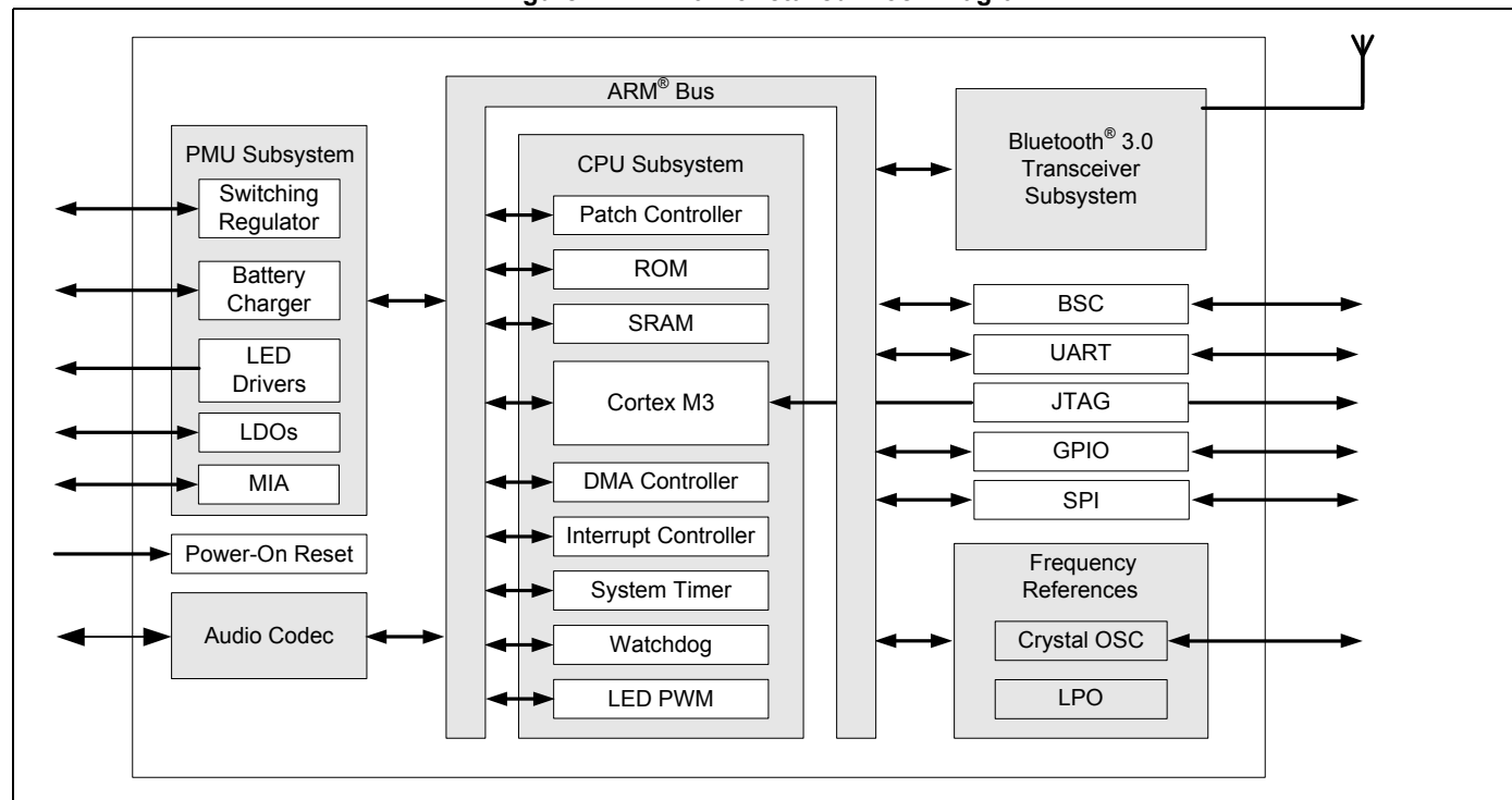
Figure 2. CYW20745 Detailed Block Diagram
