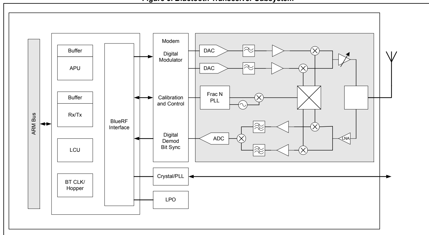
Figure 3. Bluetooth Transceiver Subsystem
