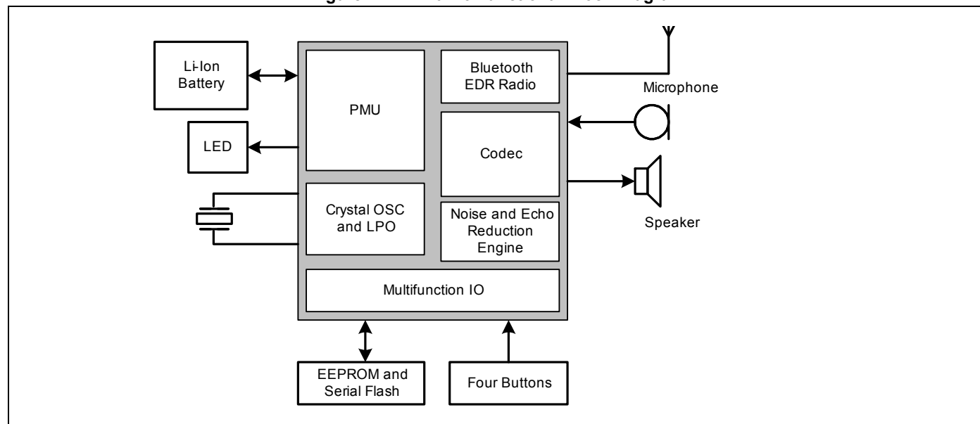
Figure 1. CYW20745 Functional Block Diagram
