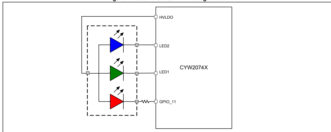
Figure 4. Recommended LED Configuration 6
