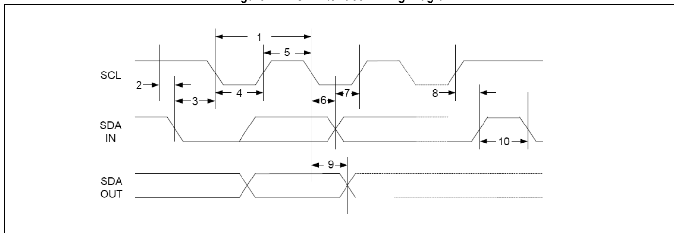
Figure 11. BSC Interface Timing Diagram
