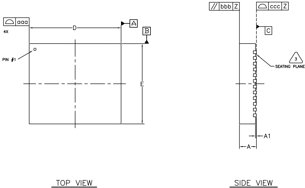
Figure 12. CYW20745, 8.0 mm × 7.0 mm, 52-Pin QFN Package Outline Drawing
