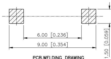
PCB.WELDING DRAWING
