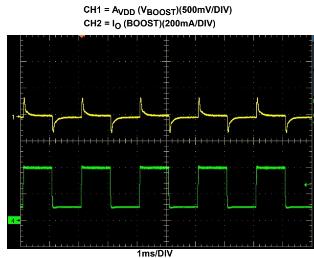
FIGURE 10. BOOST TRANSIENT RESPONSE
