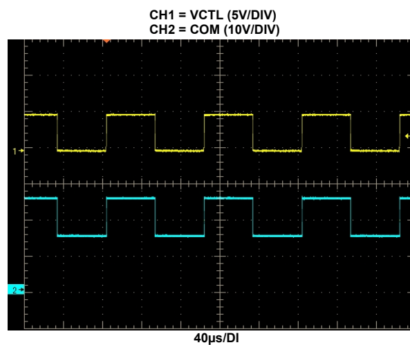
FIGURE 12. V_{ON} SLICE OPERATION
