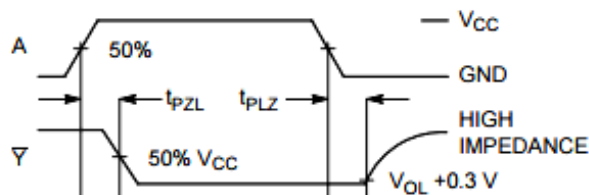
Figure 3. Switching Waveforms
