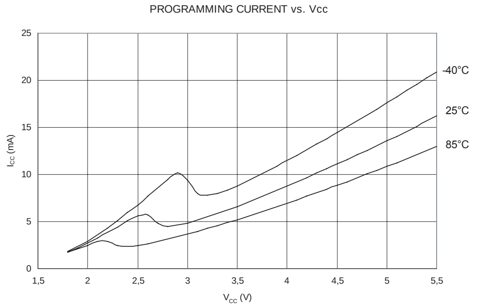
Figure 201. Programming Current vs. V_{CC}
