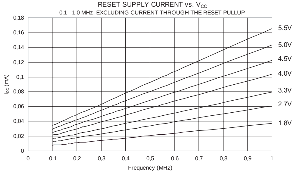
Figure 202. Reset Supply Current vs. V_{CC} (0.1 - 1.0MHz, Excluding Current Through The Reset Pullup)
