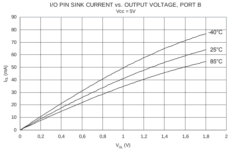
Figure 173. I/O Pin Sink Current vs. Output Voltage, Port B ( V_{CC} = 5V )
