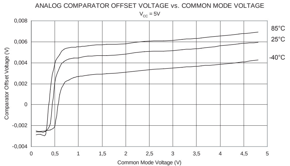
Figure 189. Analog Comparator Offset Voltage vs. Common Mode Voltage ( V_{CC} = 5V )
