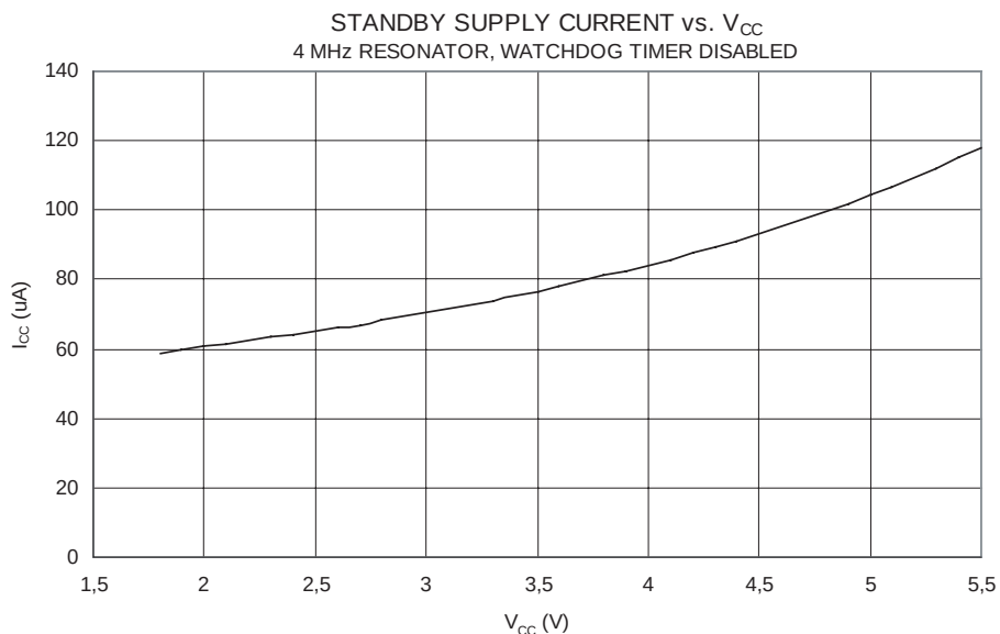
Figure 154. Standby Supply Current vs. V_{CC} (4MHz Resonator, Watchdog Timer disabled)
