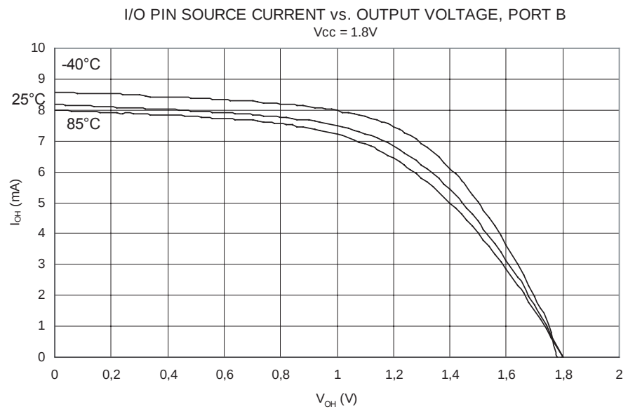
Figure 169. I/O Pin Source Current vs. Output Voltage, Port B ( V_{CC} = 1.8V )
