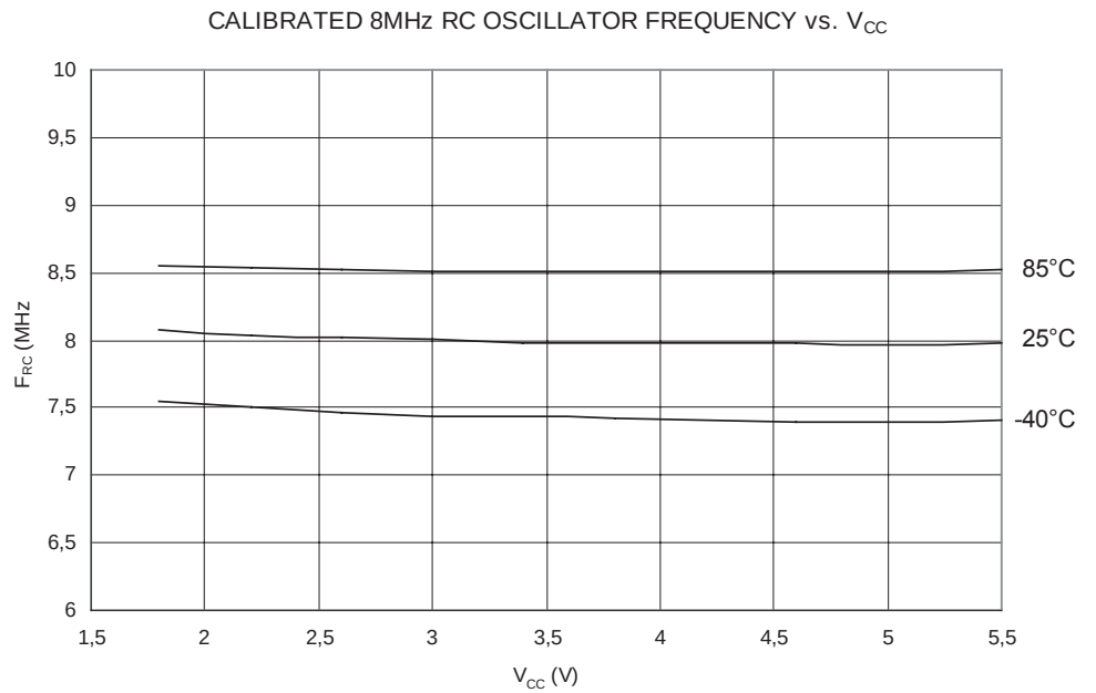
Figure 193. Calibrated 8MHz RC Oscillator Frequency vs. V_{CC}
