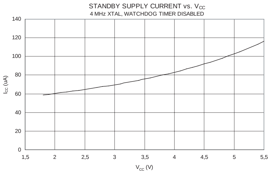
Figure 155. Standby Supply Current vs. V_{CC} (4MHz Xtal, Watchdog Timer disabled)
