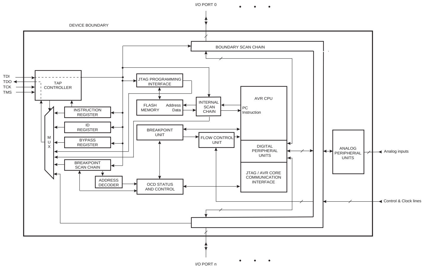
Figure 104. Block Diagram
