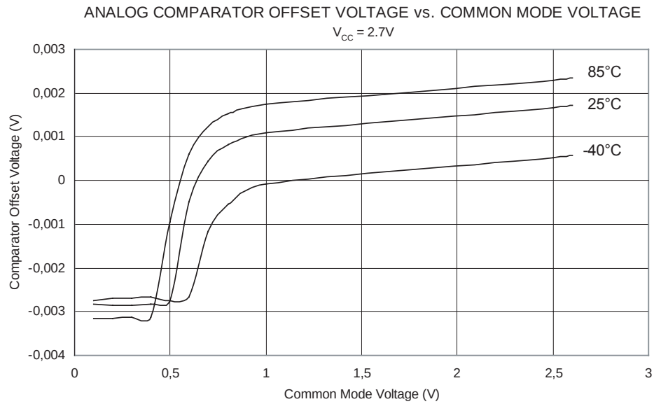
Figure 190. Analog Comparator Offset Voltage vs. Common Mode Voltage ( V_{CC} = 2.7V )
