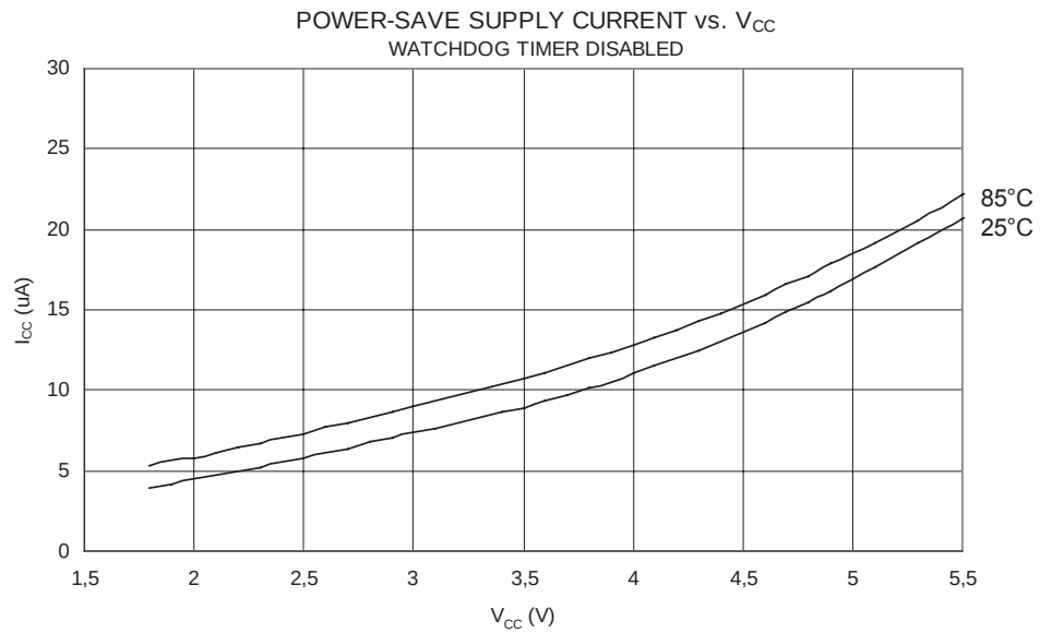
Figure 149. Power-Save Supply Current vs. V_{CC} (Watchdog Timer disabled)
