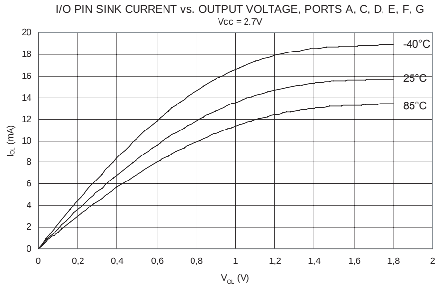
Figure 171. I/O Pin Sink Current vs. Output Voltage, Ports A, C, D, E, F, G ( V_{CC} = 2.7V )
