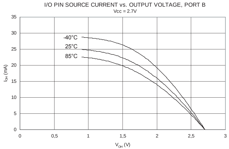
Figure 168. I/O Pin Source Current vs. Output Voltage, Port B ( V_{CC} = 2.7V )
