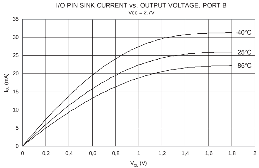
Figure 174. I/O Pin Sink Current vs. Output Voltage, Port B ( V_{CC} = 2.7V )
