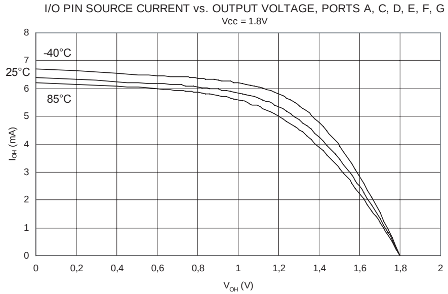
Figure 166. I/O Pin Source Current vs. Output Voltage, Ports A, C, D, E, F, G ( V_{CC} = 1.8V )
