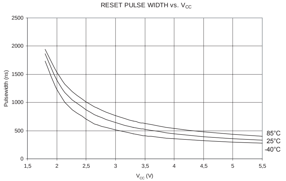
Figure 204. Reset Pulse Width vs V_{CC}
