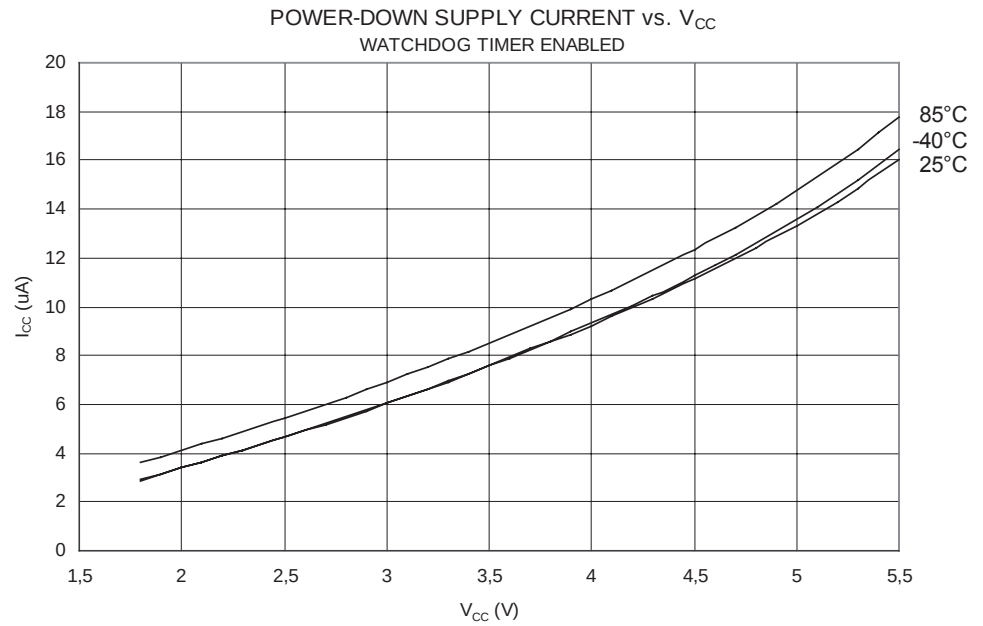
Figure 148. Power-Down Supply Current vs. V_{CC} (Watchdog Timer enabled)
