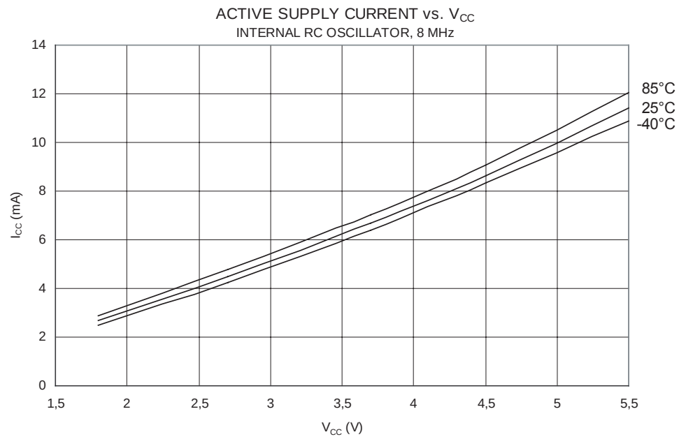
Figure 139. Active Supply Current vs. V_{CC} (Internal RC Oscillator, 8Mhz)
