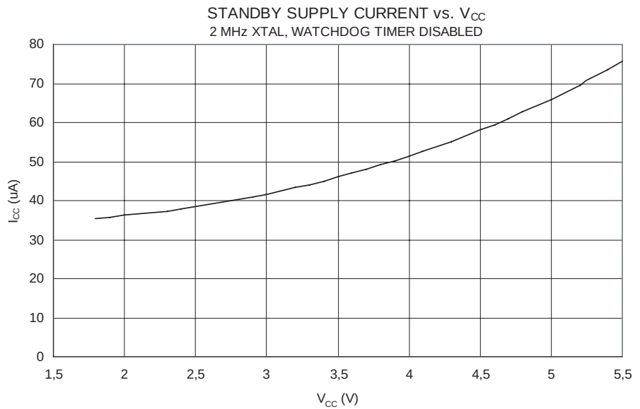
Figure 153. Standby Supply Current vs. V_{CC} (2MHz Xtal, Watchdog Timer disabled)
