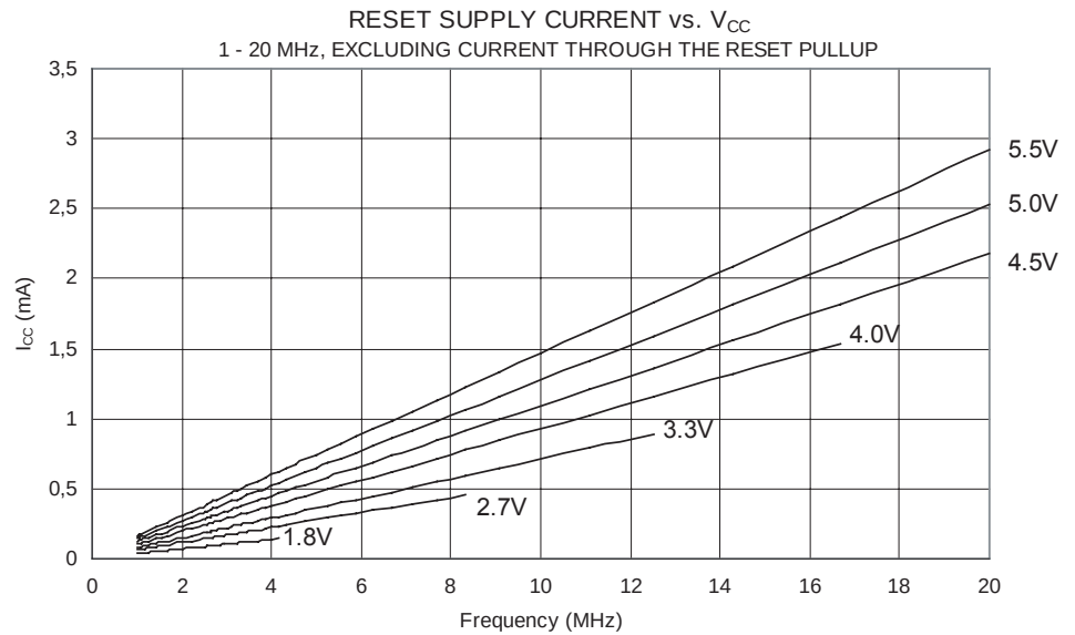
Figure 203. Reset Supply Current vs. V_{CC} (1 - 20MHz, Excluding Current Through The Reset Pullup)
