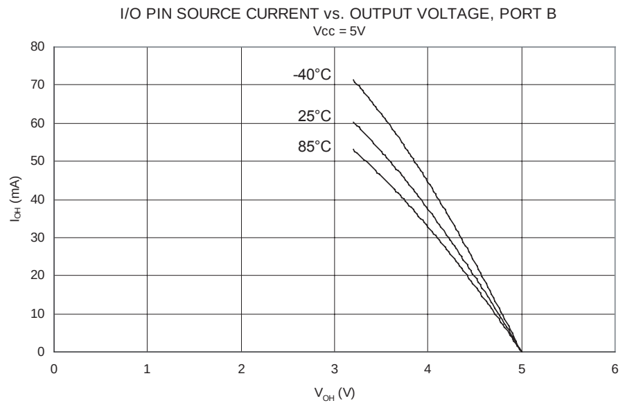
Figure 167. I/O Pin Source Current vs. Output Voltage, Port B ( V_{CC} = 5V )
