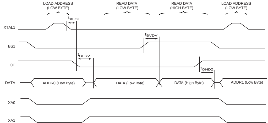
Figure 126. Parallel Programming Timing, Reading Sequence (within the Same Page) with Timing Requirements (1)
