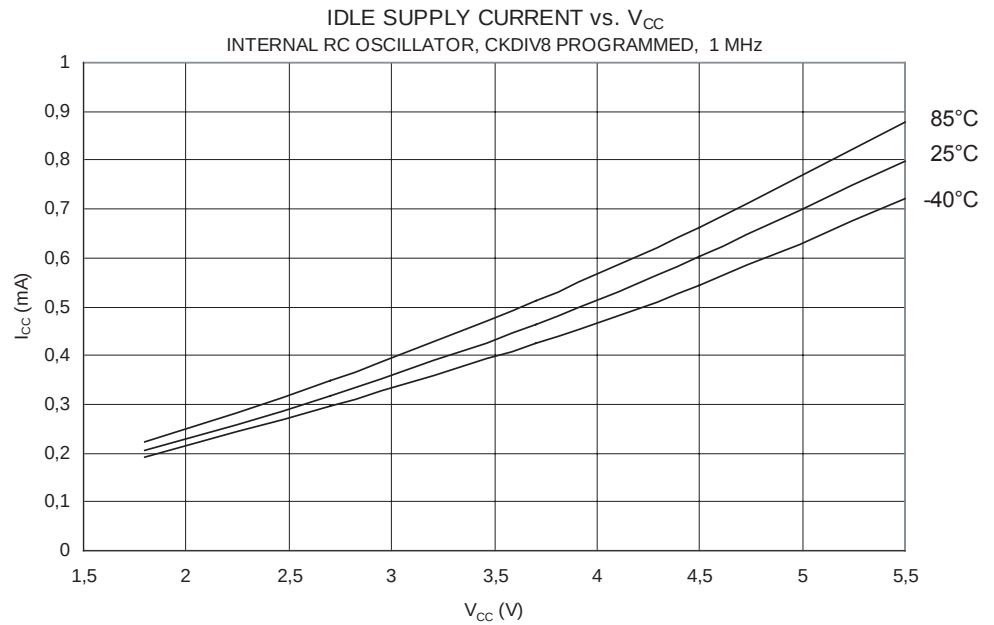
Figure 145. Idle Supply Current vs. V_{CC} (Internal RC Oscillator, CKDIV8 programmed, 1MHz)
