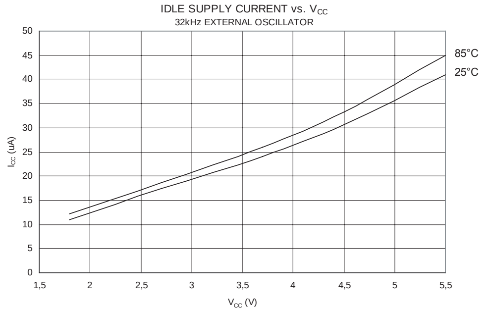
Figure 146. Idle Supply Current vs. V_{CC} (32kHz External Oscillator)
