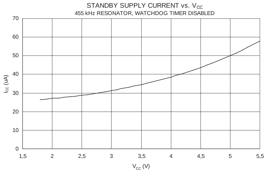
Figure 150. Standby Supply Current vs. V_{CC} (455kHz Resonator, Watchdog Timer disabled)
