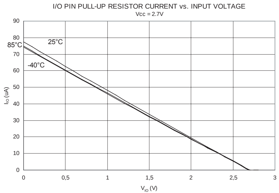
Figure 159. I/O Pin Pull-up Resistor Current vs. Input Voltage ( V_{CC} = 2.7V )
