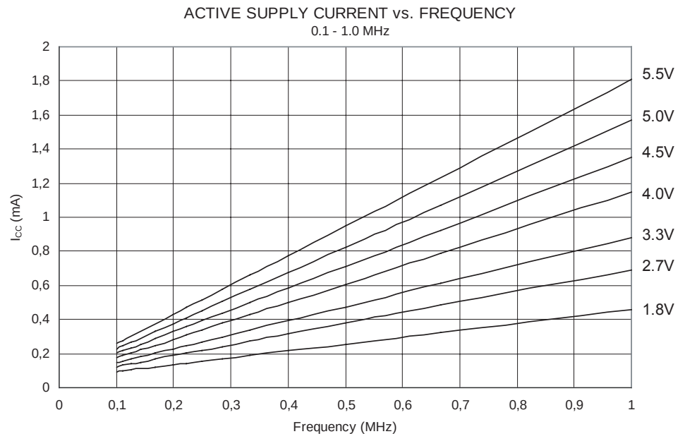
Figure 137. Active Supply Current vs. Frequency (0.1-1.0 MHz)
