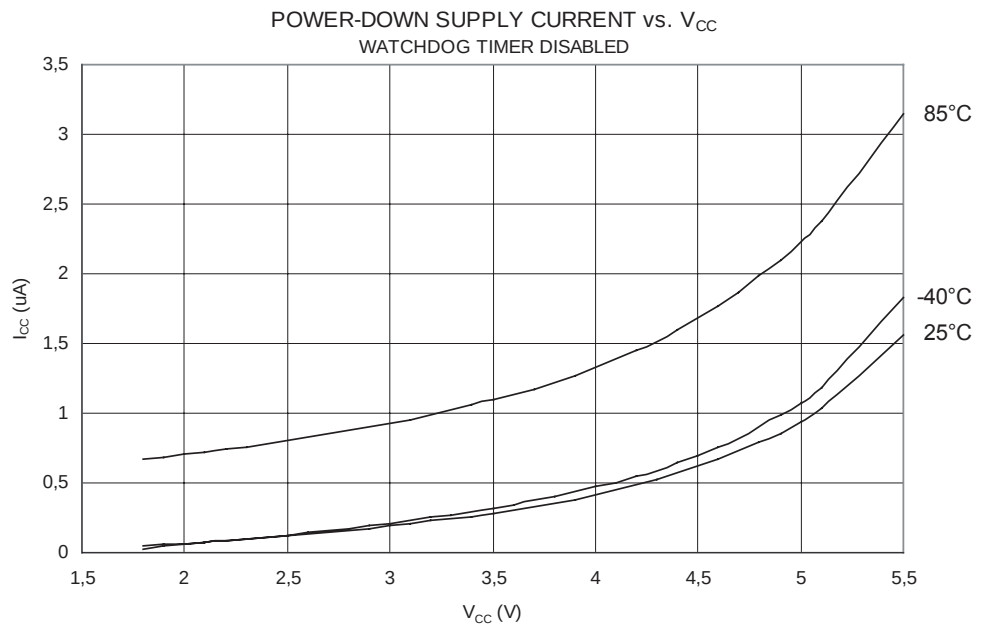
Figure 147. Power-Down Supply Current vs. V_{CC} (Watchdog Timer disabled)
