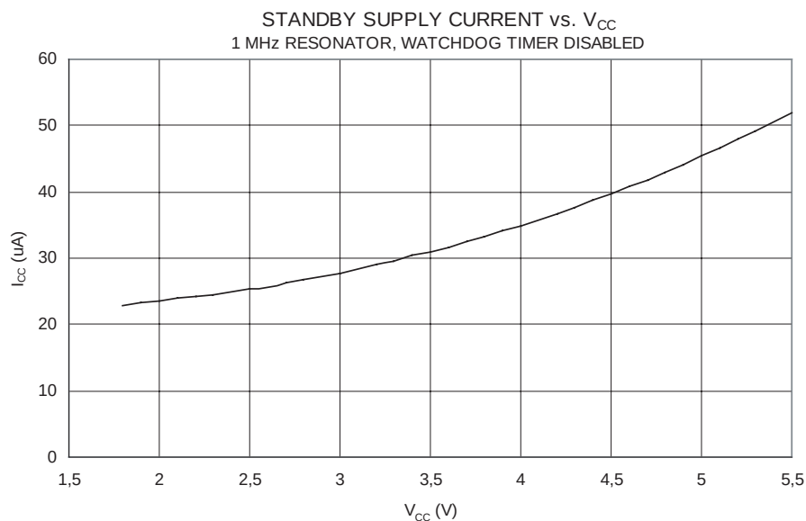
Figure 151. Standby Supply Current vs. V_{CC} (1MHz Resonator, Watchdog Timer disabled)
