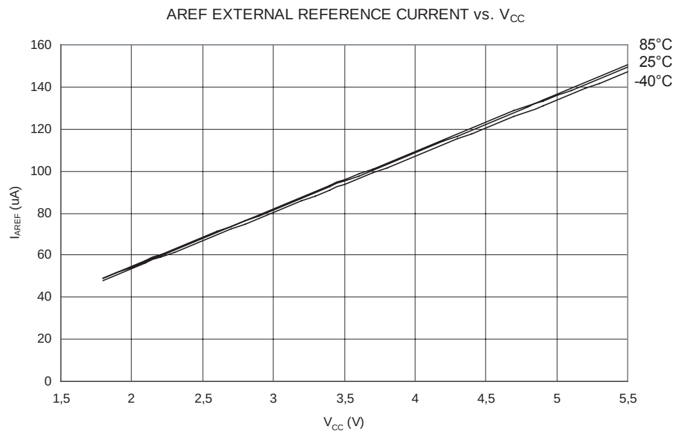
Figure 197. A_{REF} External Reference Current vs. V_{CC}
