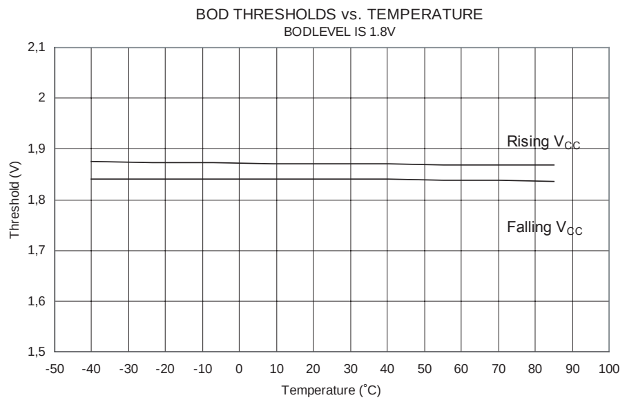
Figure 187. BOD Thresholds vs. Temperature (BOD Level is 1.8V)
