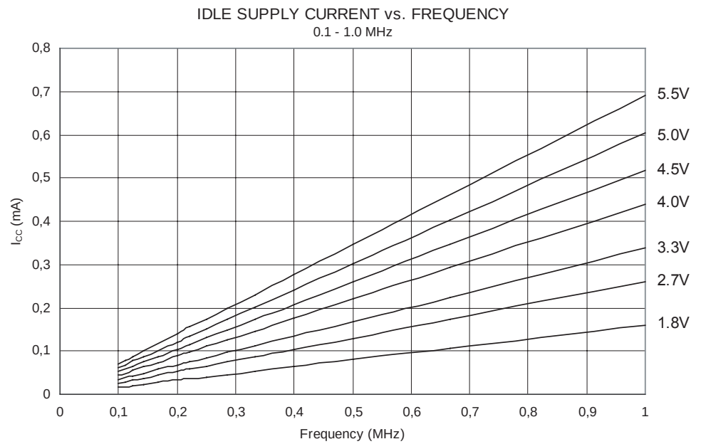
Figure 142. Idle Supply Current vs. Frequency (0.1-1.0 MHz)
