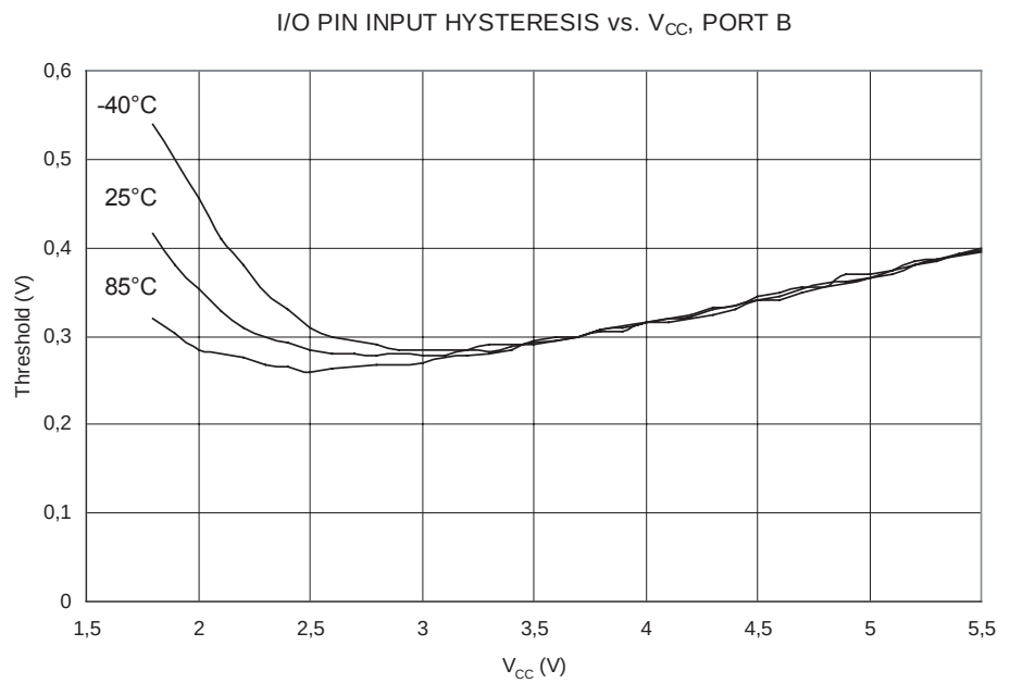
Figure 181. I/O Pin Input Hysteresis vs. V_{CC} , Port B
