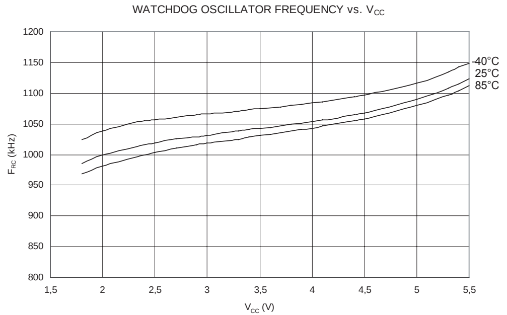
Figure 191. Watchdog Oscillator Frequency vs. V_{CC}
