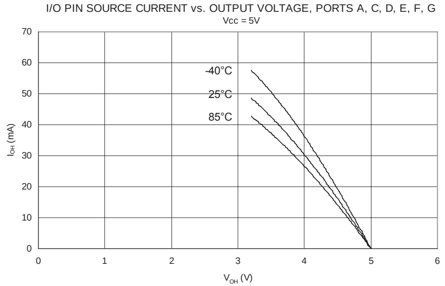
Figure 164. I/O Pin Source Current vs. Output Voltage, Ports A, C, D, E, F, G ( V_{CC} = 5V )
