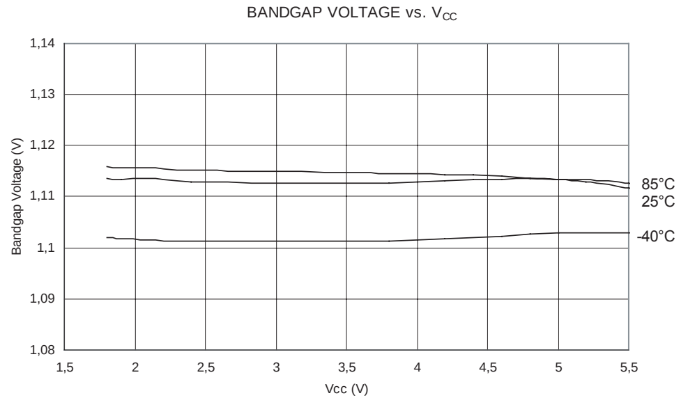
Figure 188. Bandgap Voltage vs. V_{CC}
