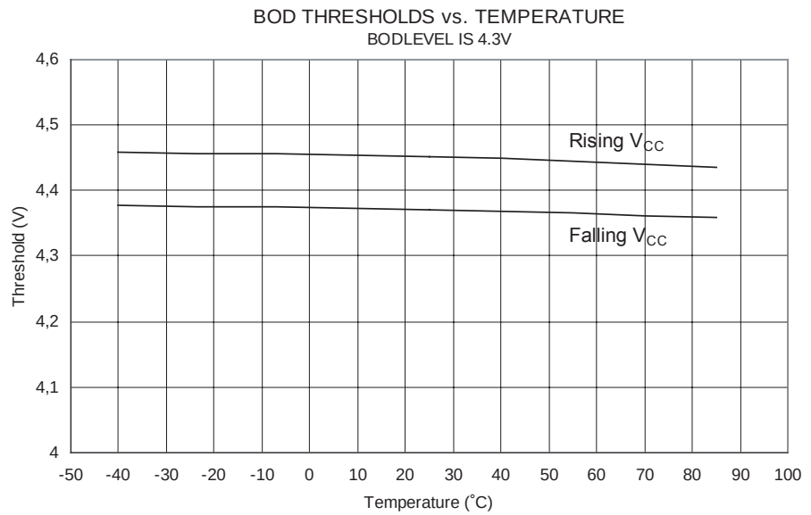
Figure 185. BOD Thresholds vs. Temperature (BOD Level is 4.3V)
