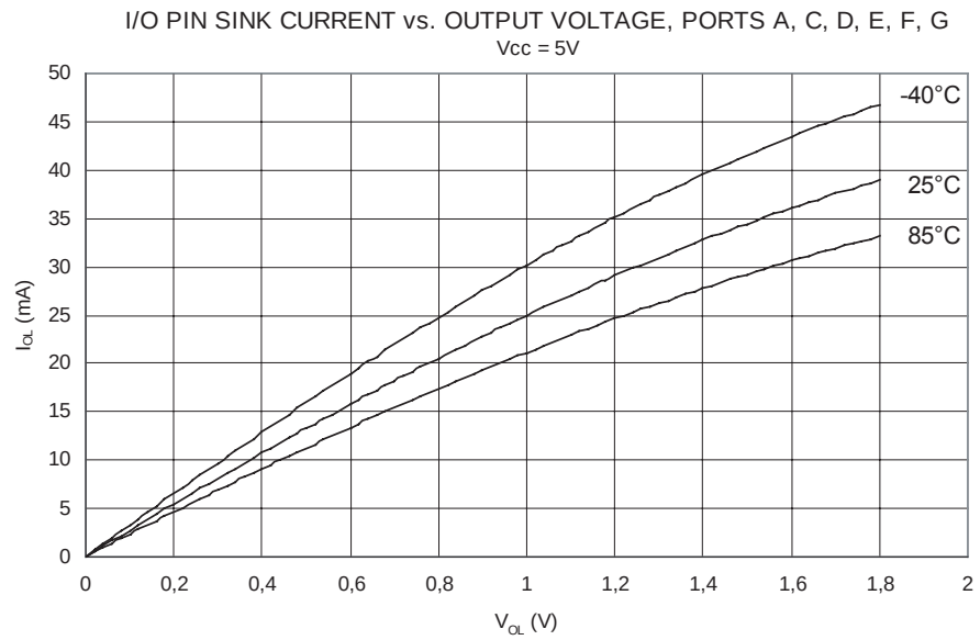
Figure 170. I/O Pin Sink Current vs. Output Voltage, Ports A, C, D, E, F, G ( V_{CC} = 5V )
