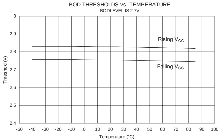
Figure 186. BOD Thresholds vs. Temperature (BOD Level is 2.7V)
