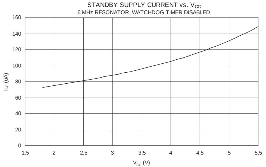
Figure 157. Standby Supply Current vs. V_{CC} (6MHz Xtal, Watchdog Timer disabled)
