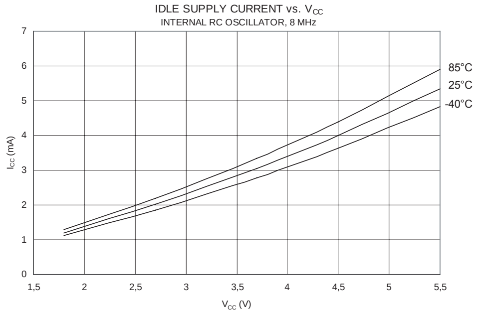
Figure 144. Idle Supply Current vs. V_{CC} (Internal RC Oscillator, 8MHz)
