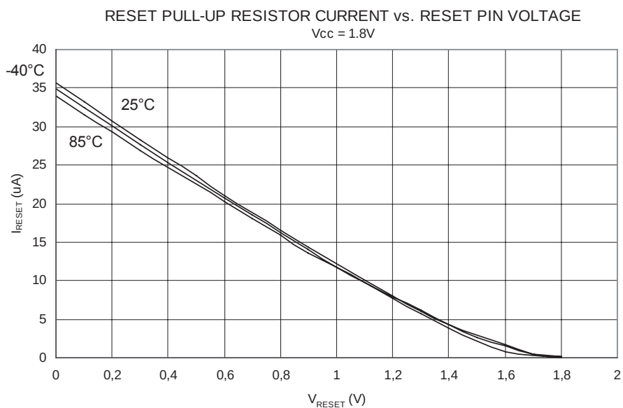
Figure 163. Reset Pull-Up Resistor Current vs. Reset Pin Voltage ( V_{CC} = 1.8V )
