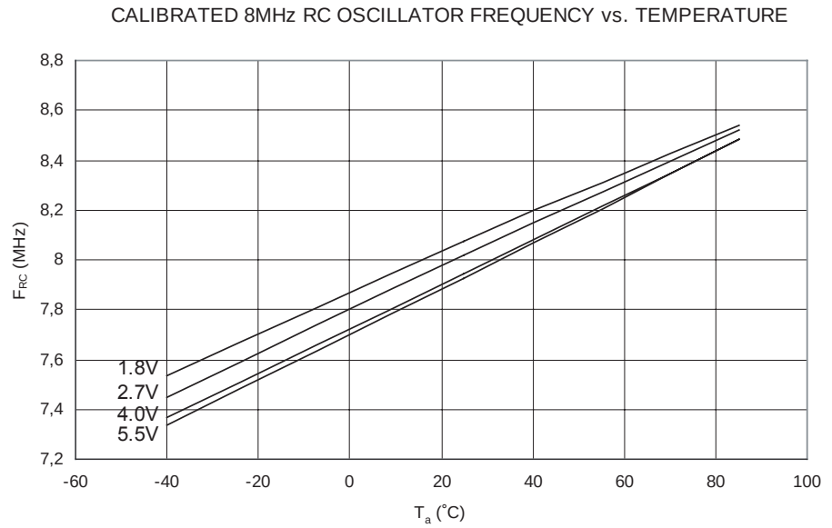
Figure 192. Calibrated 8MHz RC Oscillator Frequency vs. Temperature
