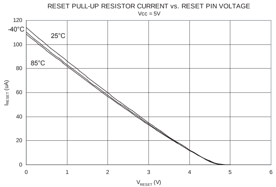
Figure 161. Reset Pull-Up Resistor Current vs. Reset Pin Voltage ( V_{CC} = 5V )
