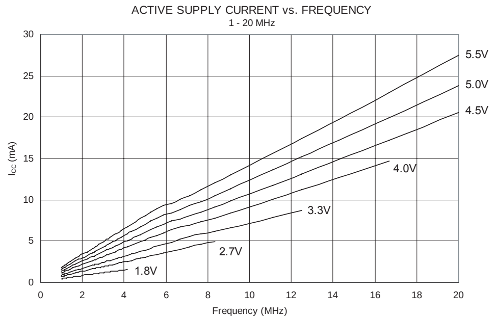
Figure 138. Active Supply Current vs. Frequency (1-20 MHz)
