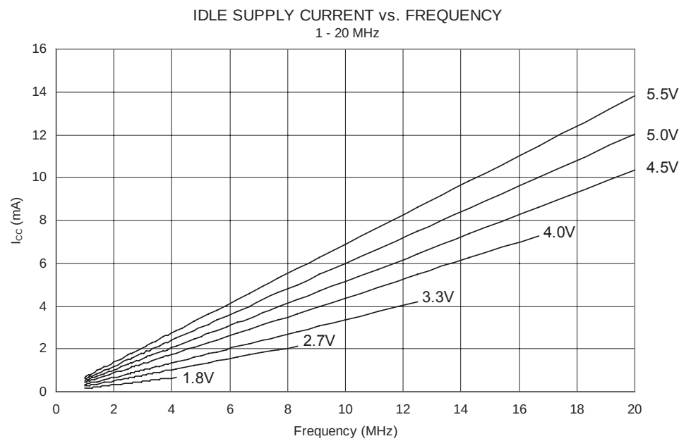
Figure 143. Idle Supply Current vs. Frequency (1-20 MHz)
