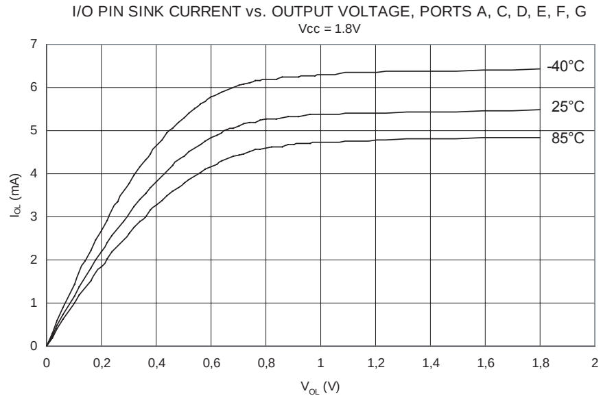
Figure 172. I/O Pin Sink Current vs. Output Voltage, Ports A, C, D, E, F, G ( V_{CC} = 1.8V )
