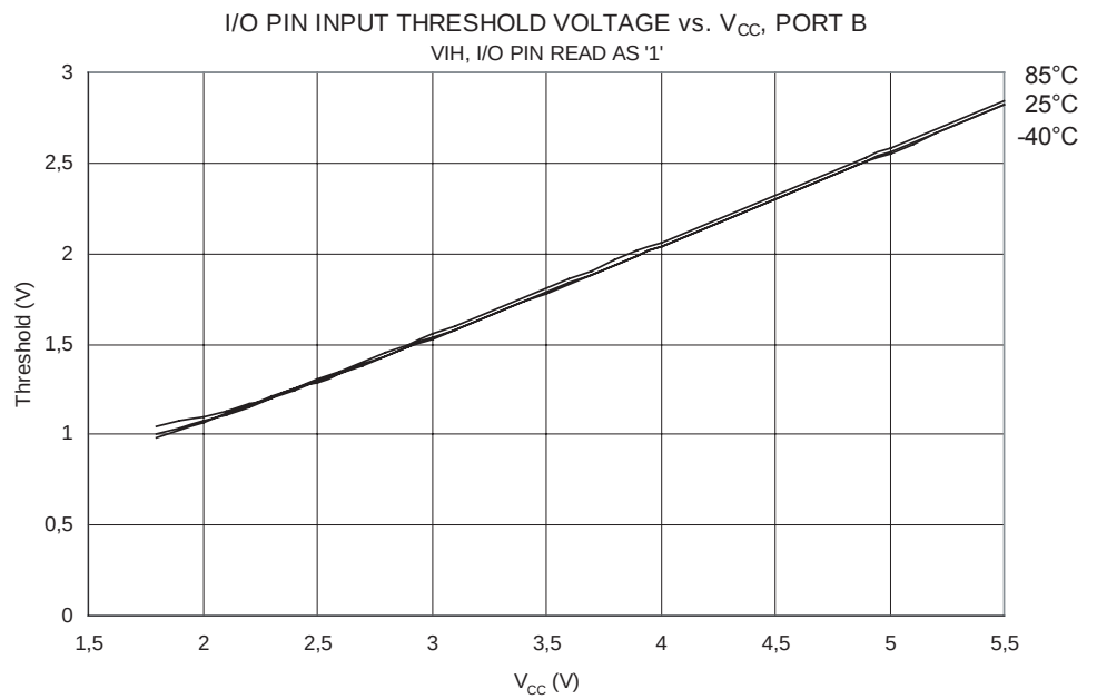
Figure 179. I/O Pin Input Threshold Voltage vs. V_{CC} , Port B ( V_{IH} , I/O Pin Read as '1')
