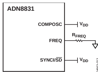
Figure 13. Free-Run Mode
