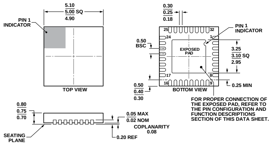
Figure 22. 32-Lead Lead Frame Chip Scale Package [LFCSP_VQ] 5 mm×5 mm Body, Very Thin Quad (CP-32-7) Dimensions Shown in Millimeters
