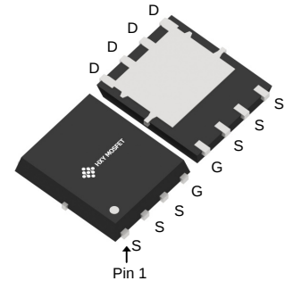
DFN5X6-8L (WPAK-8)
