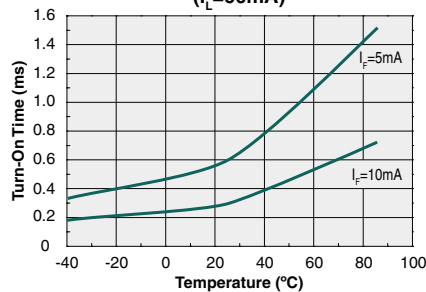
Typical Turn-On Time vs. Temperature ( I_L=60\text{mA} )
