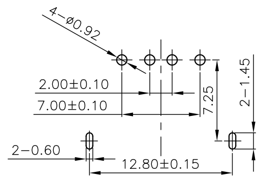
FRONT EDGE OF CONNECTOR PCB LAYOUT
