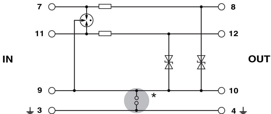
Circuit diagram
